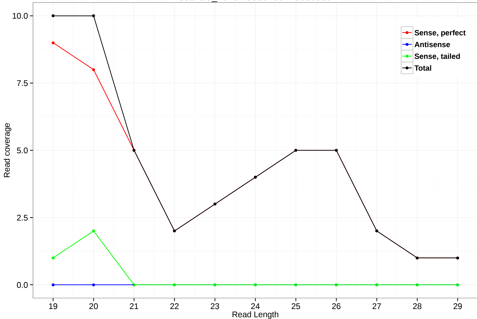
scaffold_4929:15386196-15386350
