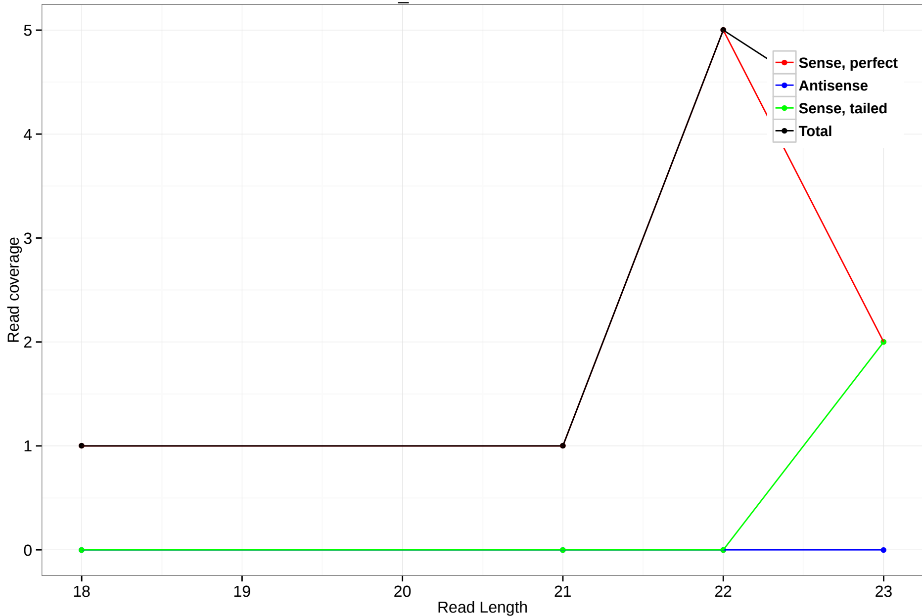
scaffold_4929:15365190-15365350
