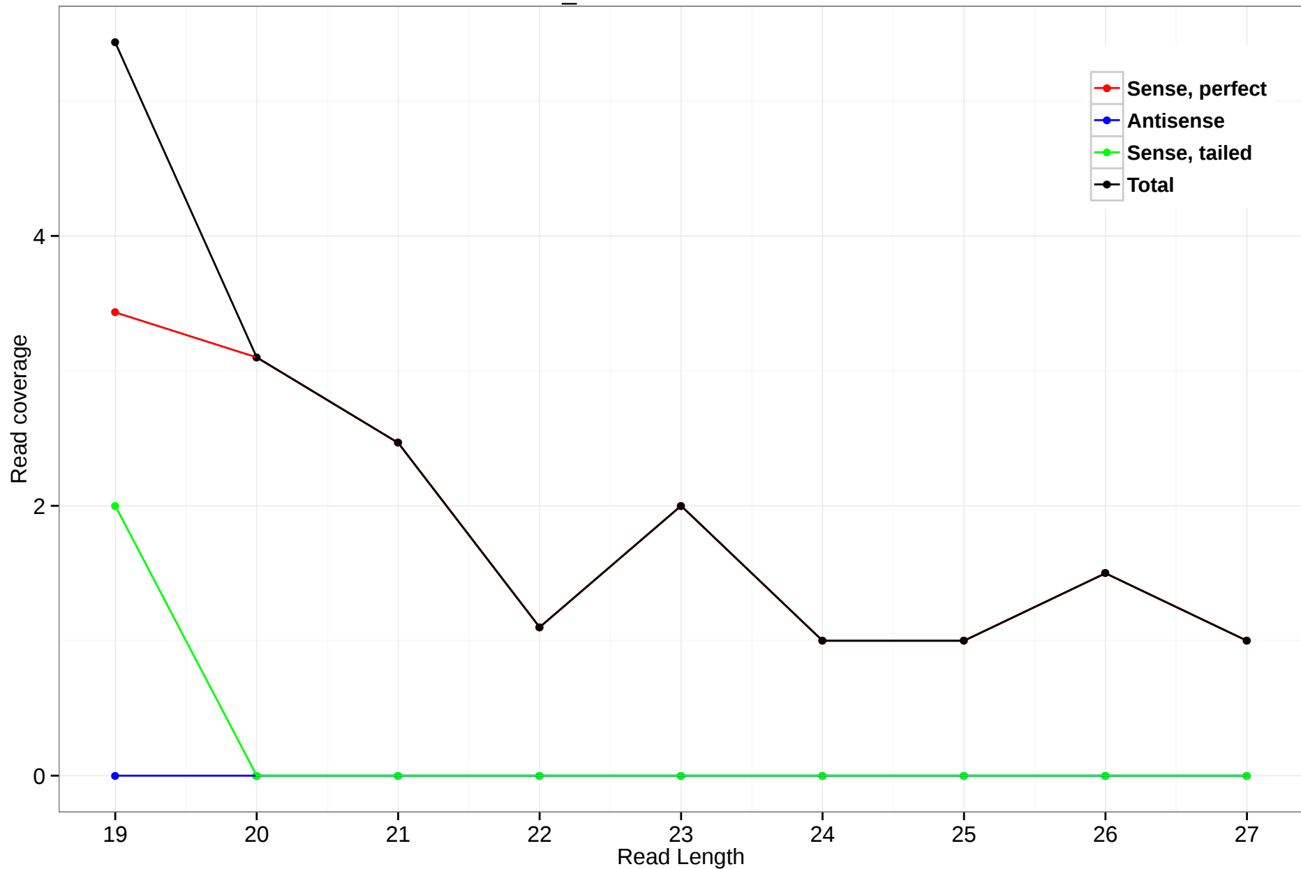
scaffold_4929:14747387-14747841
