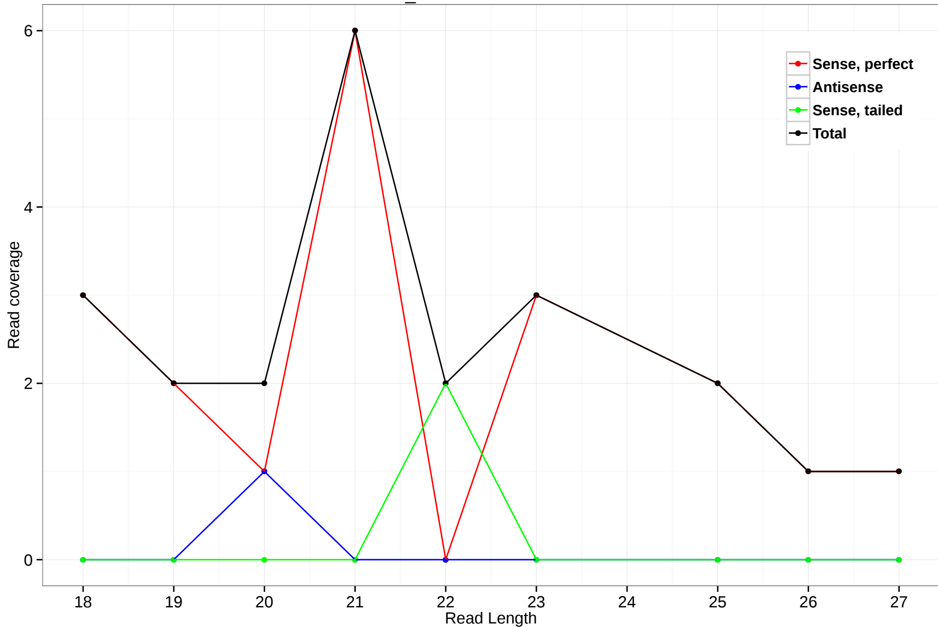
scaffold_4929:14738352-14738524
