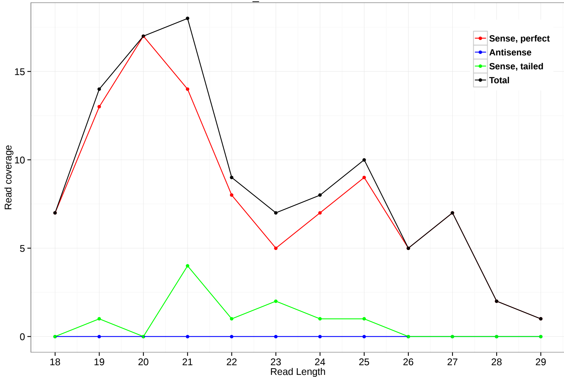
scaffold_4929:1404933-1405522
