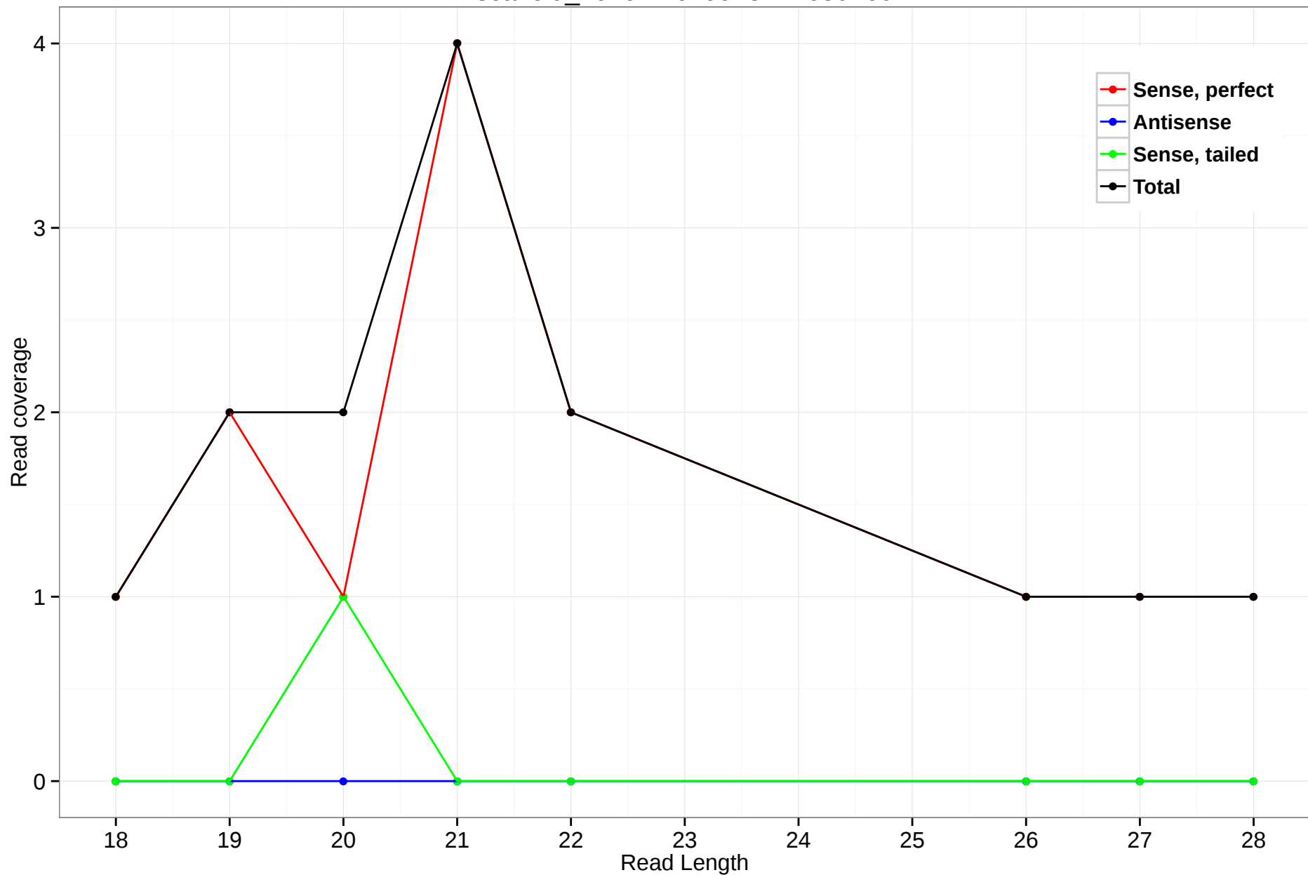
scaffold_4929:11679973-11680460
