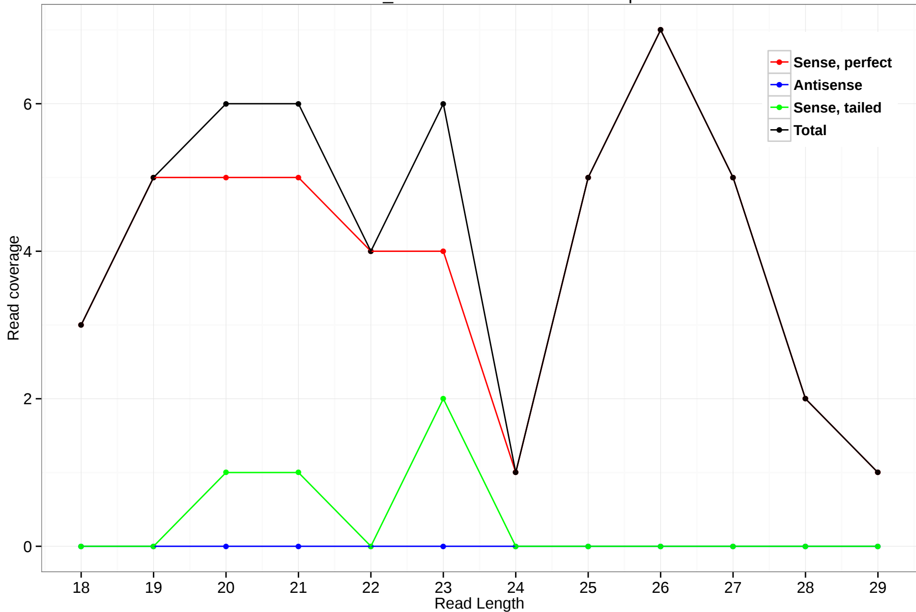
scaffold_4929:11657282-11662177.5p
