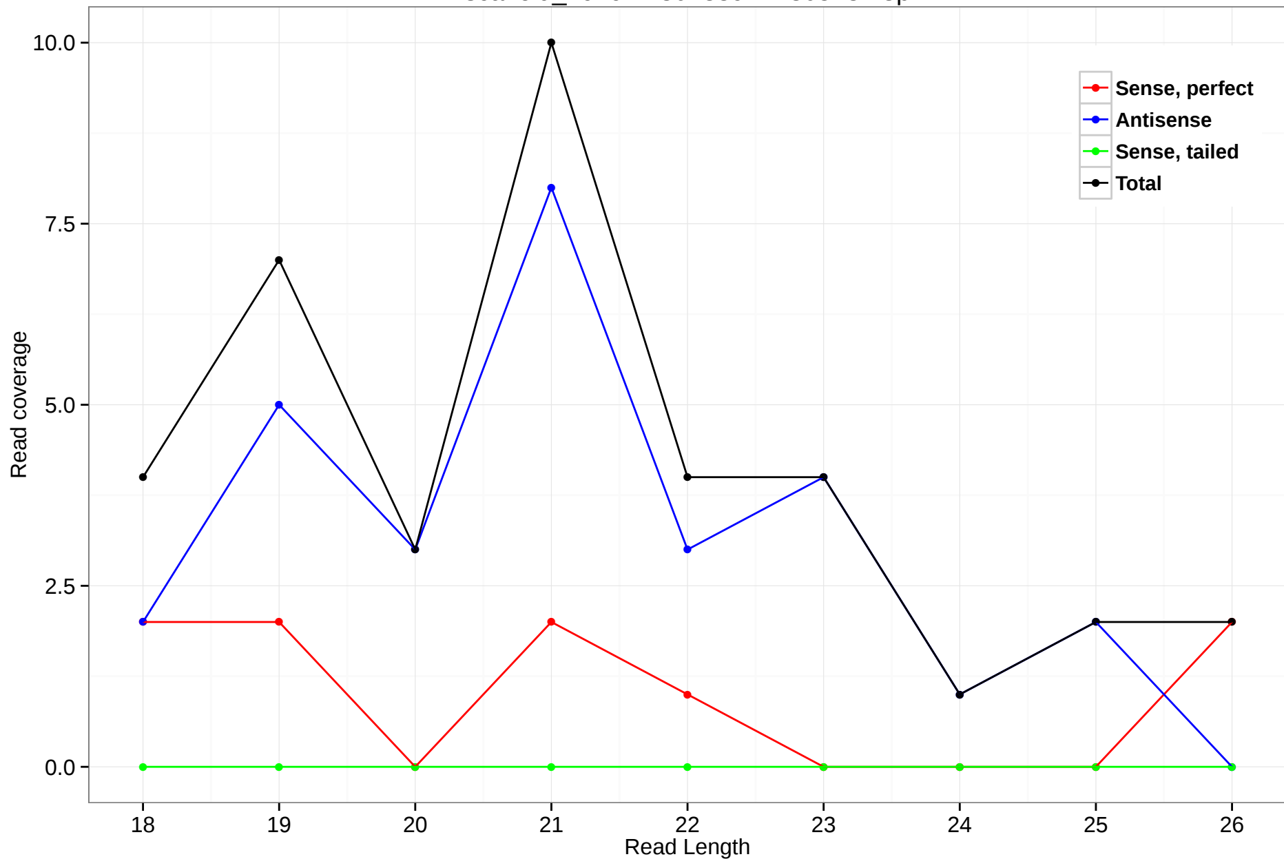
scaffold_4929:11302889-11305134.3p
