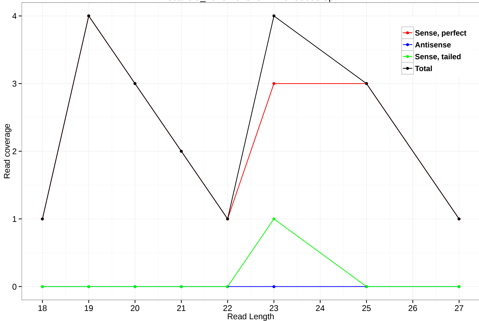
scaffold_4929:10754977-10756695.5p
