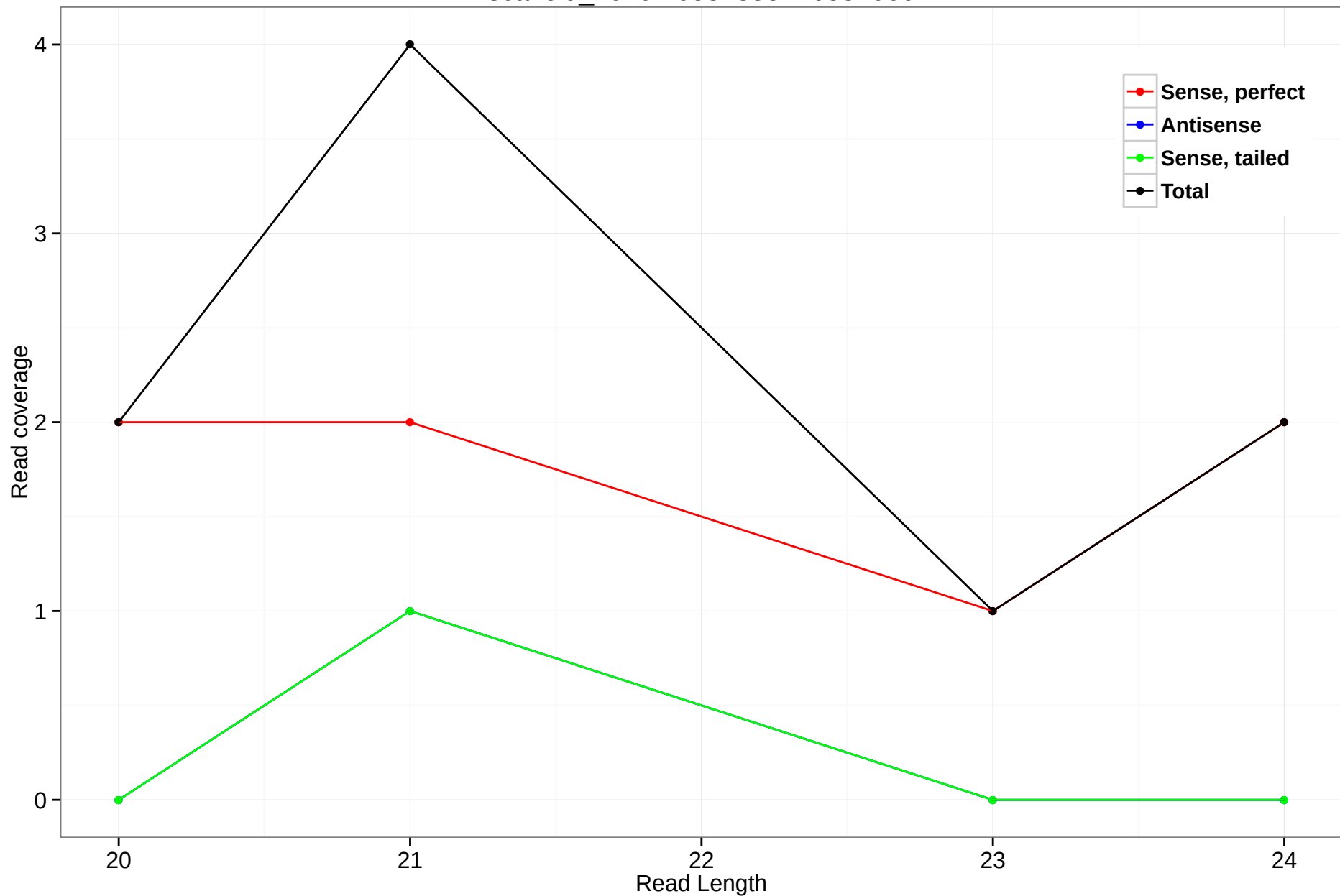
scaffold_4929:10581855-10582066
