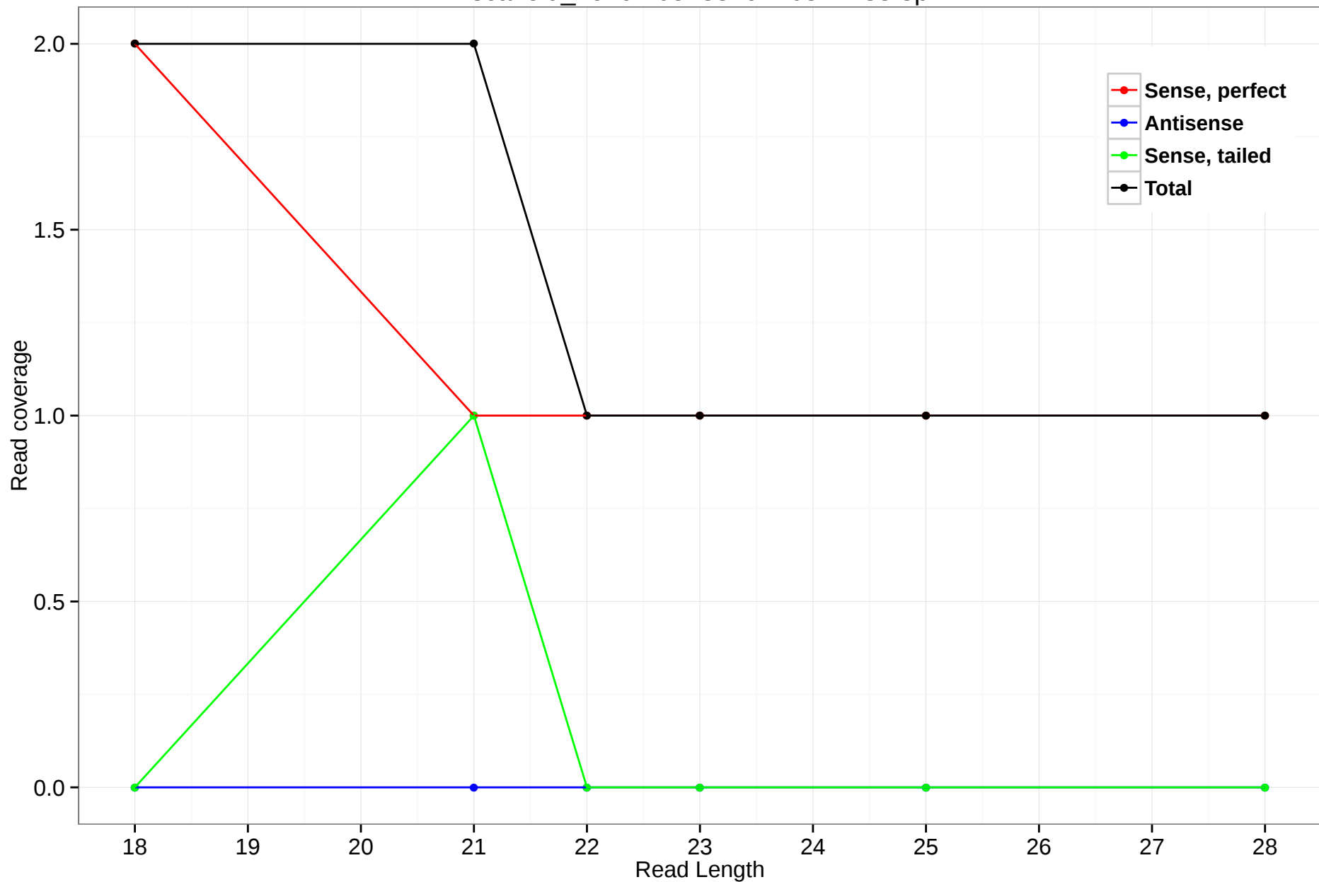
scaffold_4929:10523829-10524488.3p
