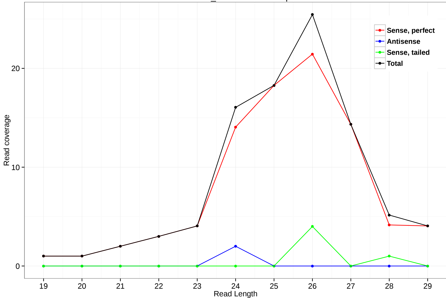
scaffold_4855:377-7853.5p
