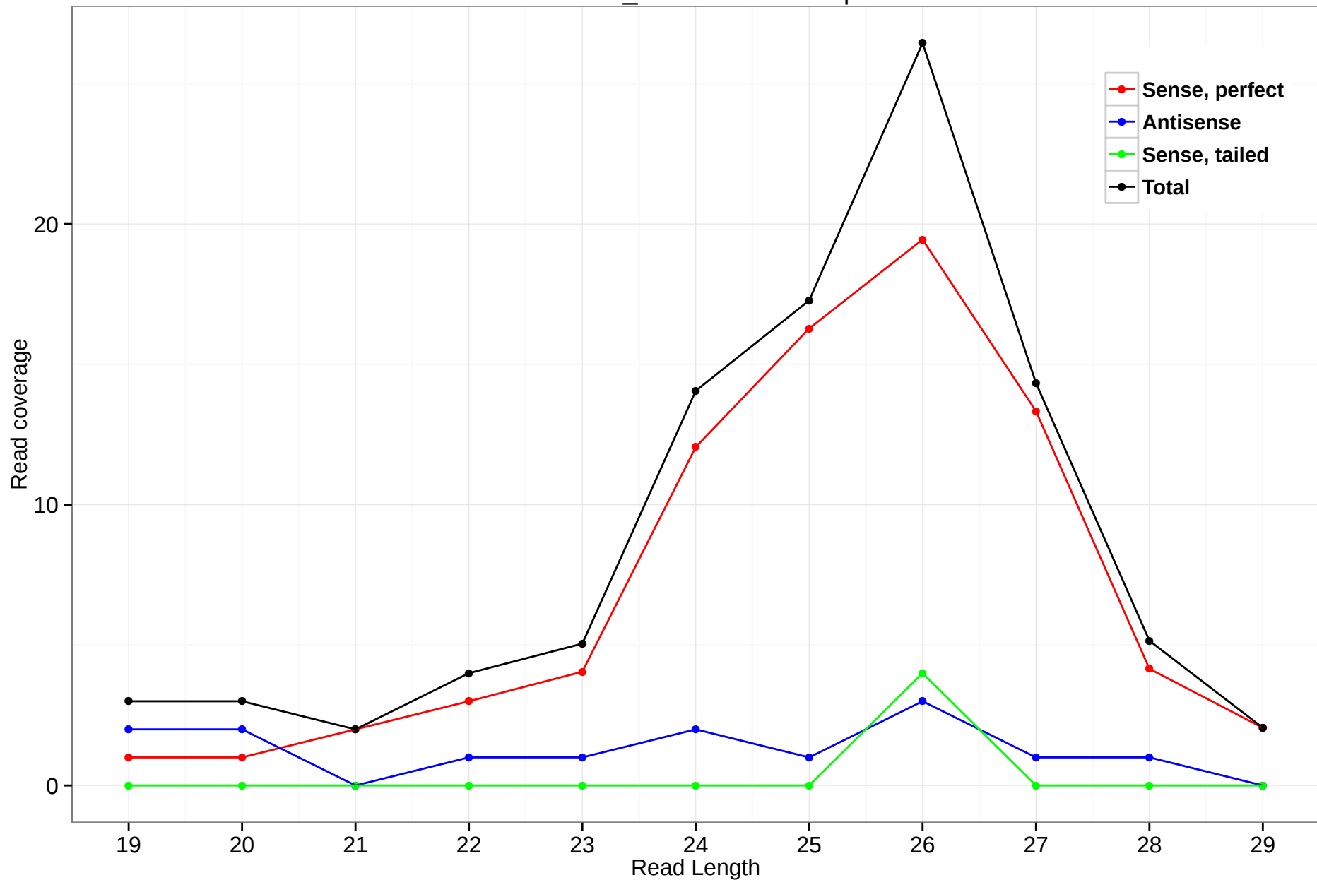
scaffold_4855:347-7865.5p
