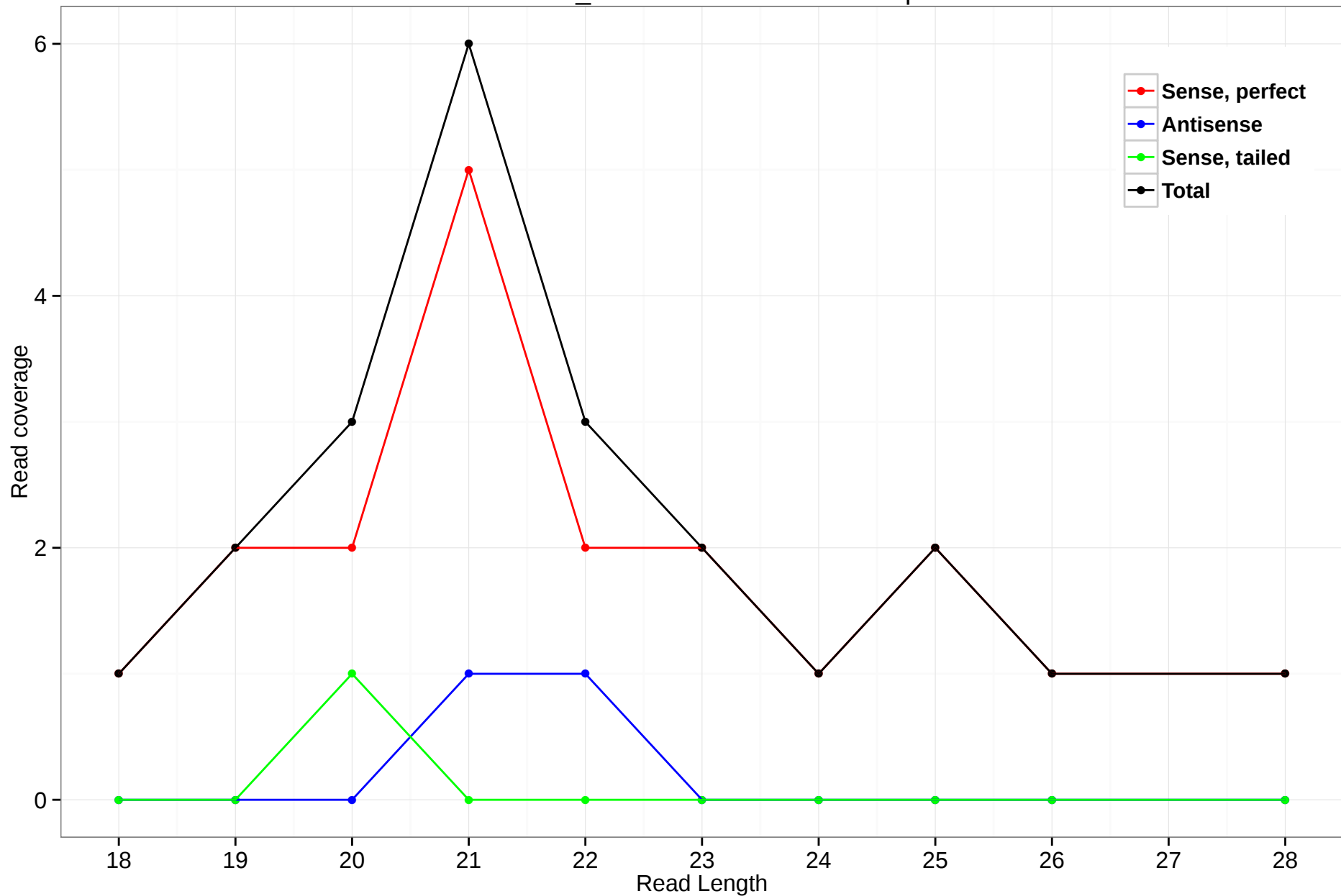
scaffold_4845:9553808-9555030.5p
