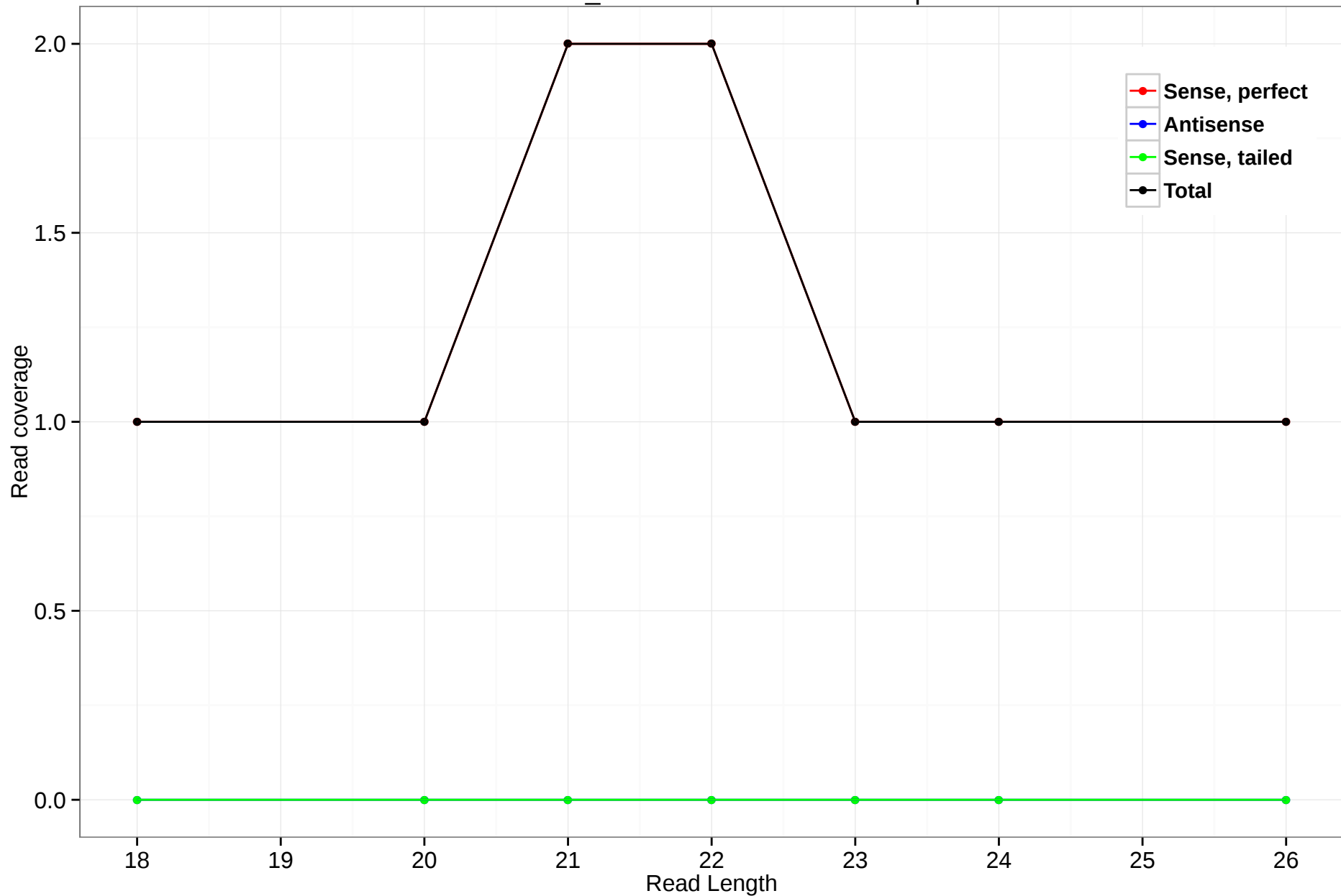
scaffold_4845:8925557-8926207.3p
