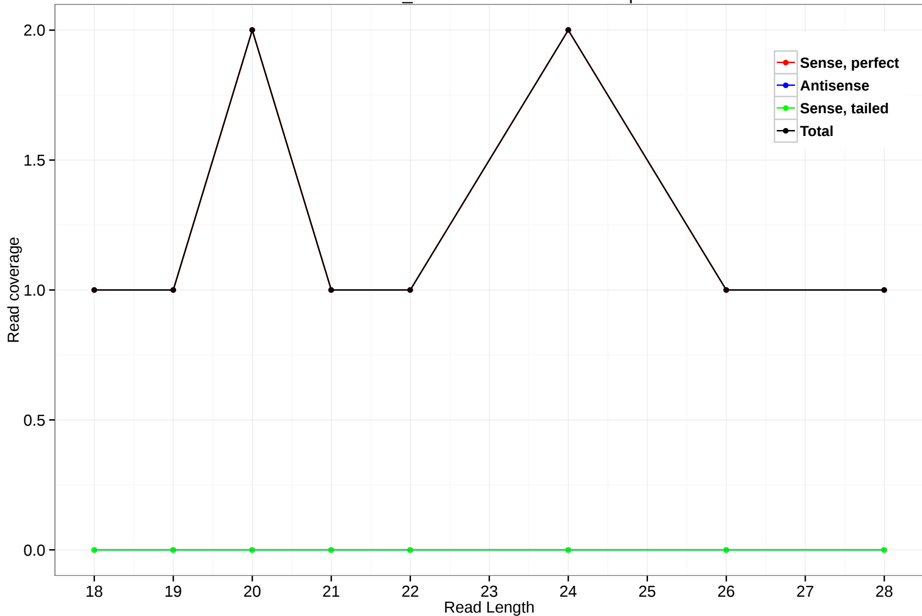
scaffold_4845:8507801-8508829.5p
