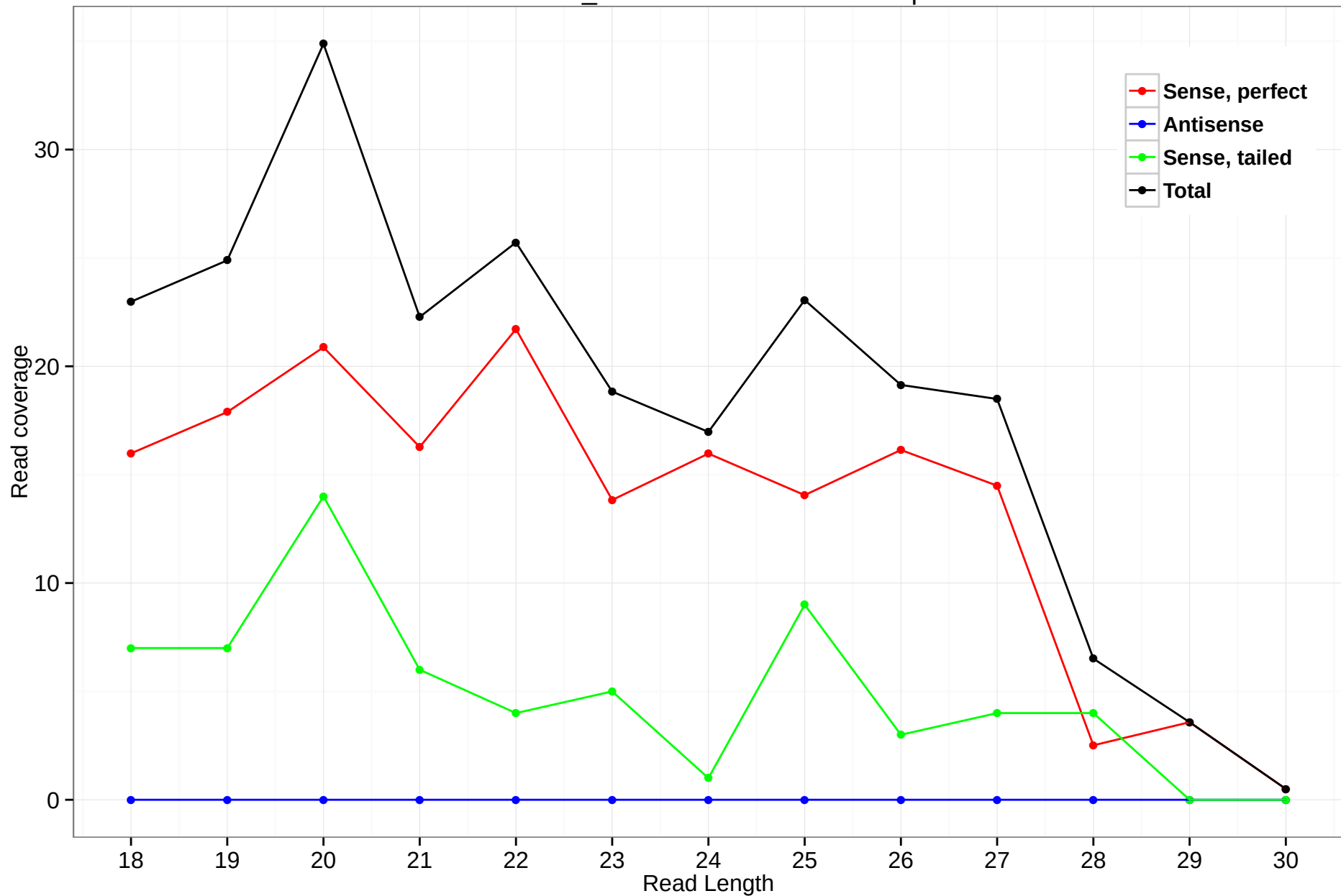
scaffold_4845:8136683-8137641.5p
