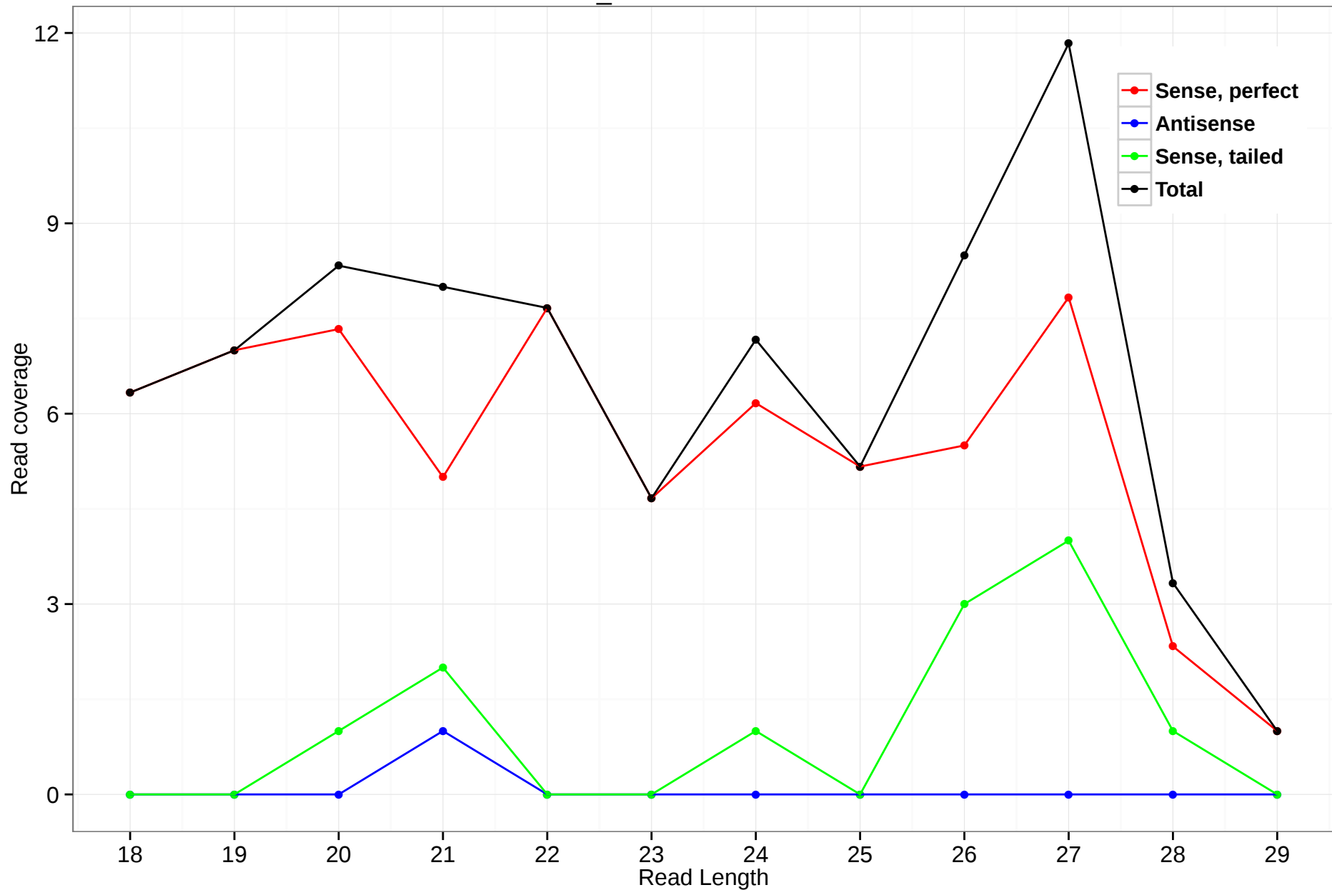
scaffold_4845:7819027-7819303
