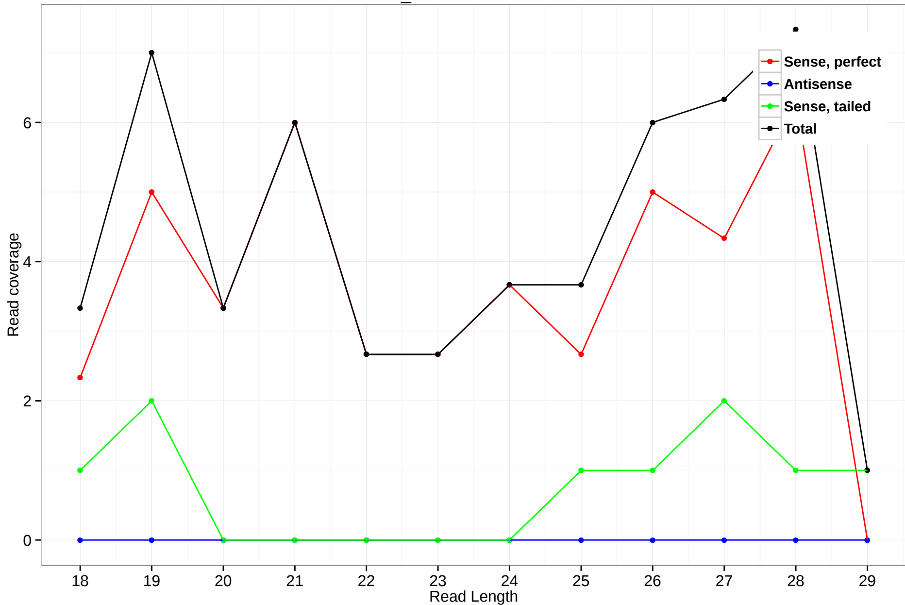
scaffold_4845:7817850-7818137
