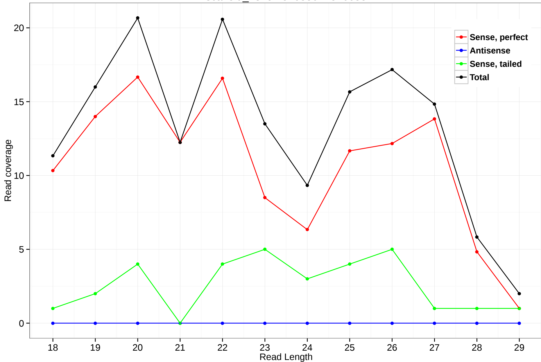
scaffold_4845:7816386-7816683
