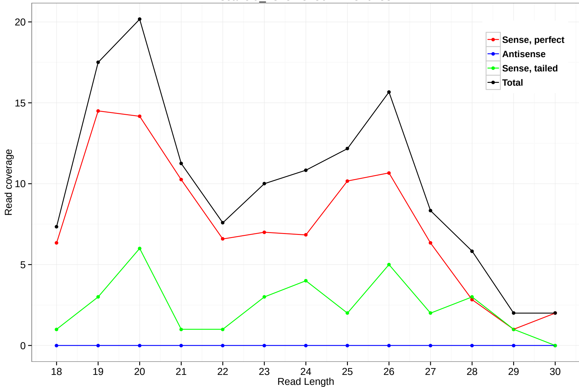
scaffold_4845:7815672-7816183
