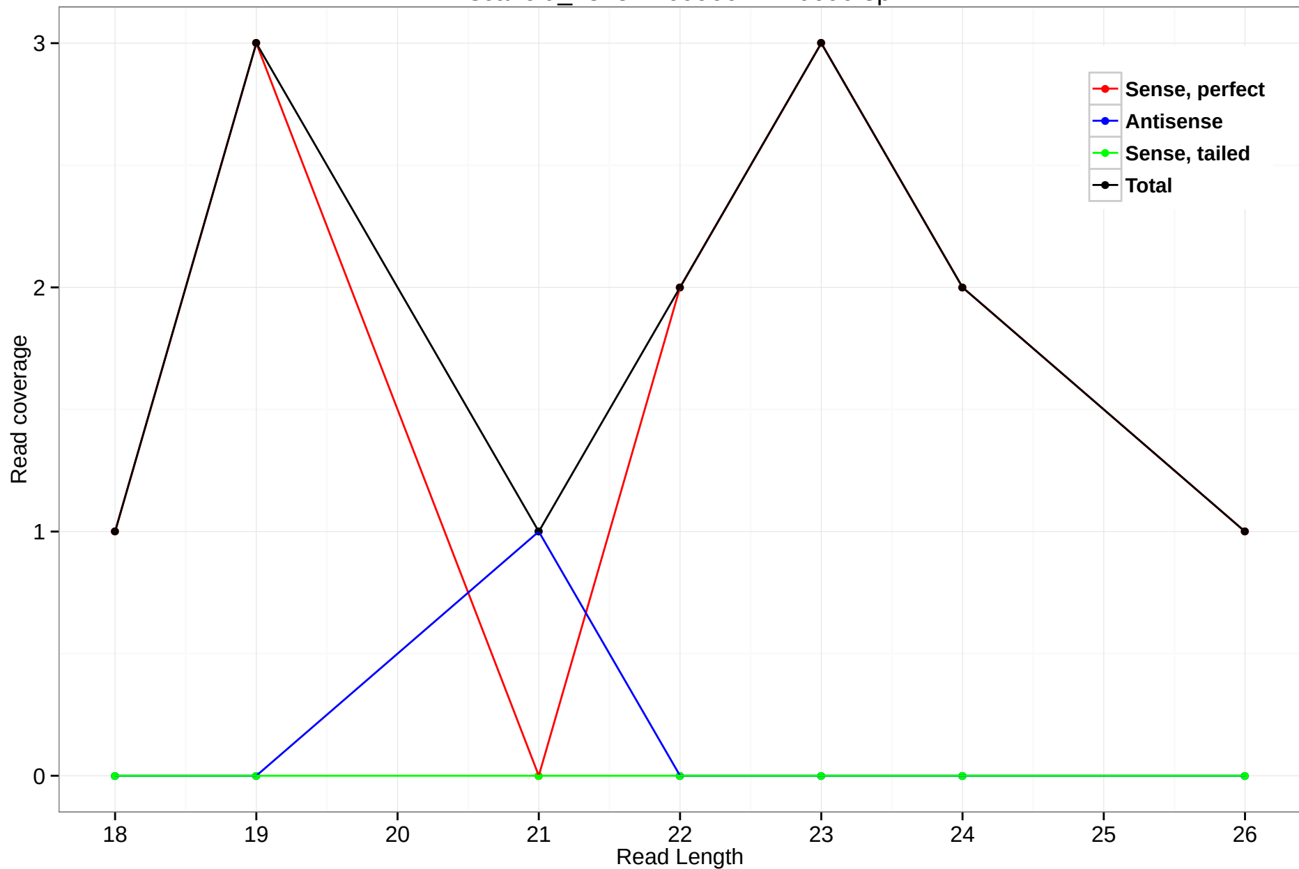
scaffold_4845:7409966-7410690.3p
