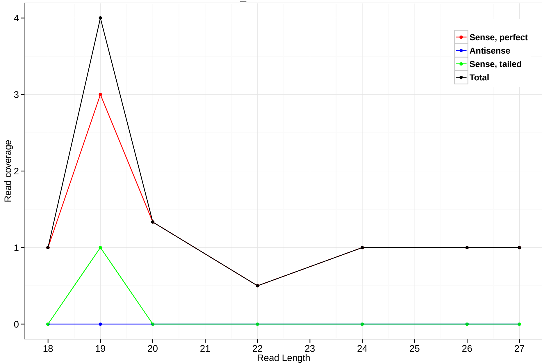
scaffold_4845:6868242-6868734
