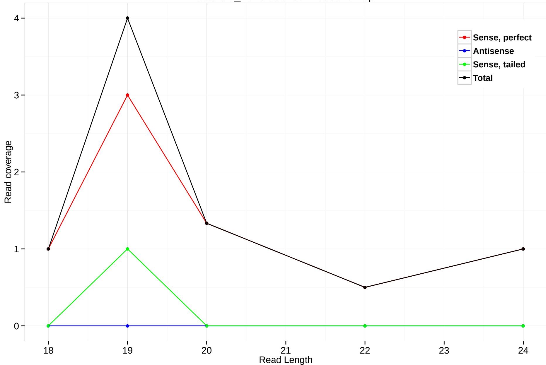
scaffold_4845:6867891-6868734.5p
