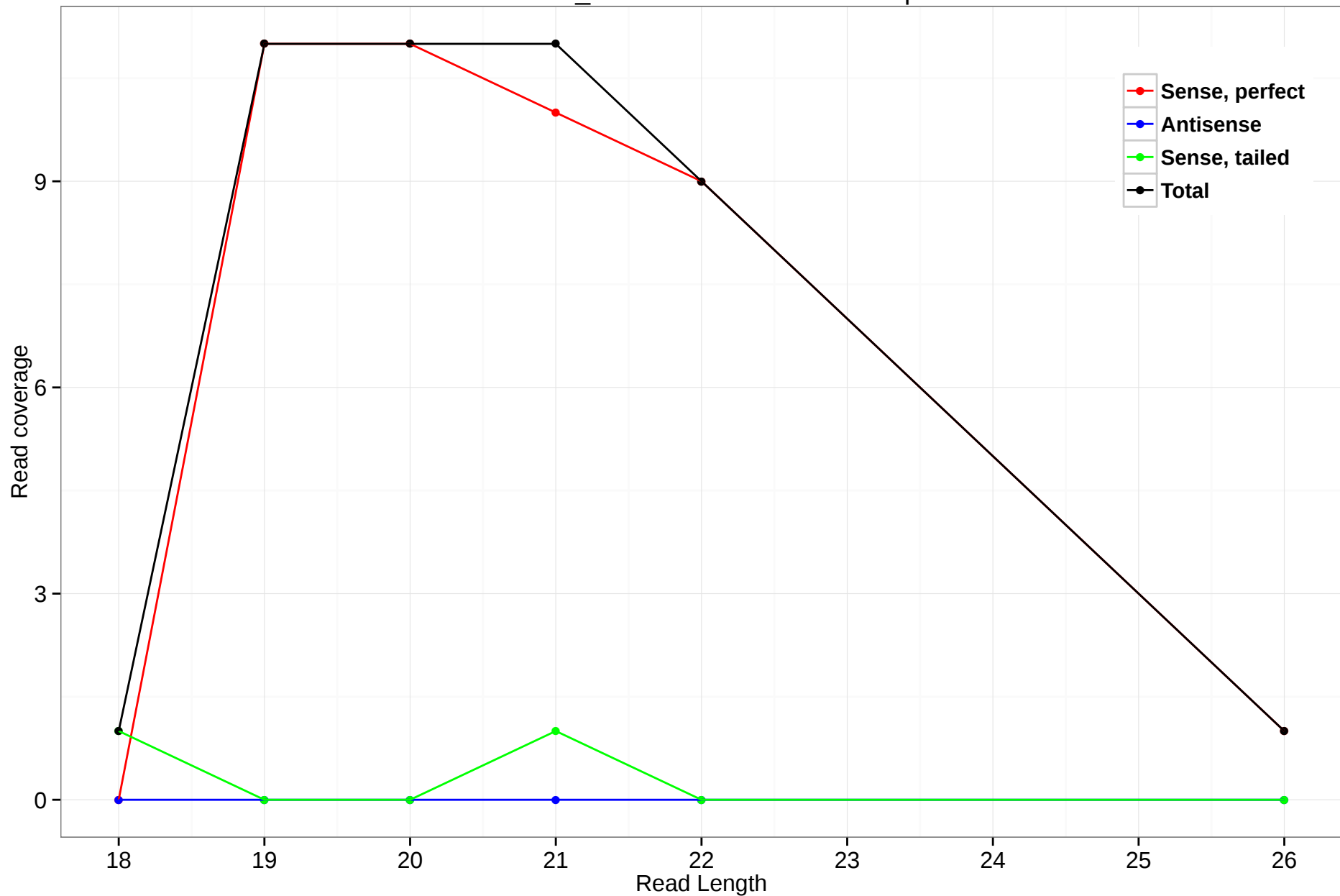
scaffold_4845:6846279-6848580.5p
