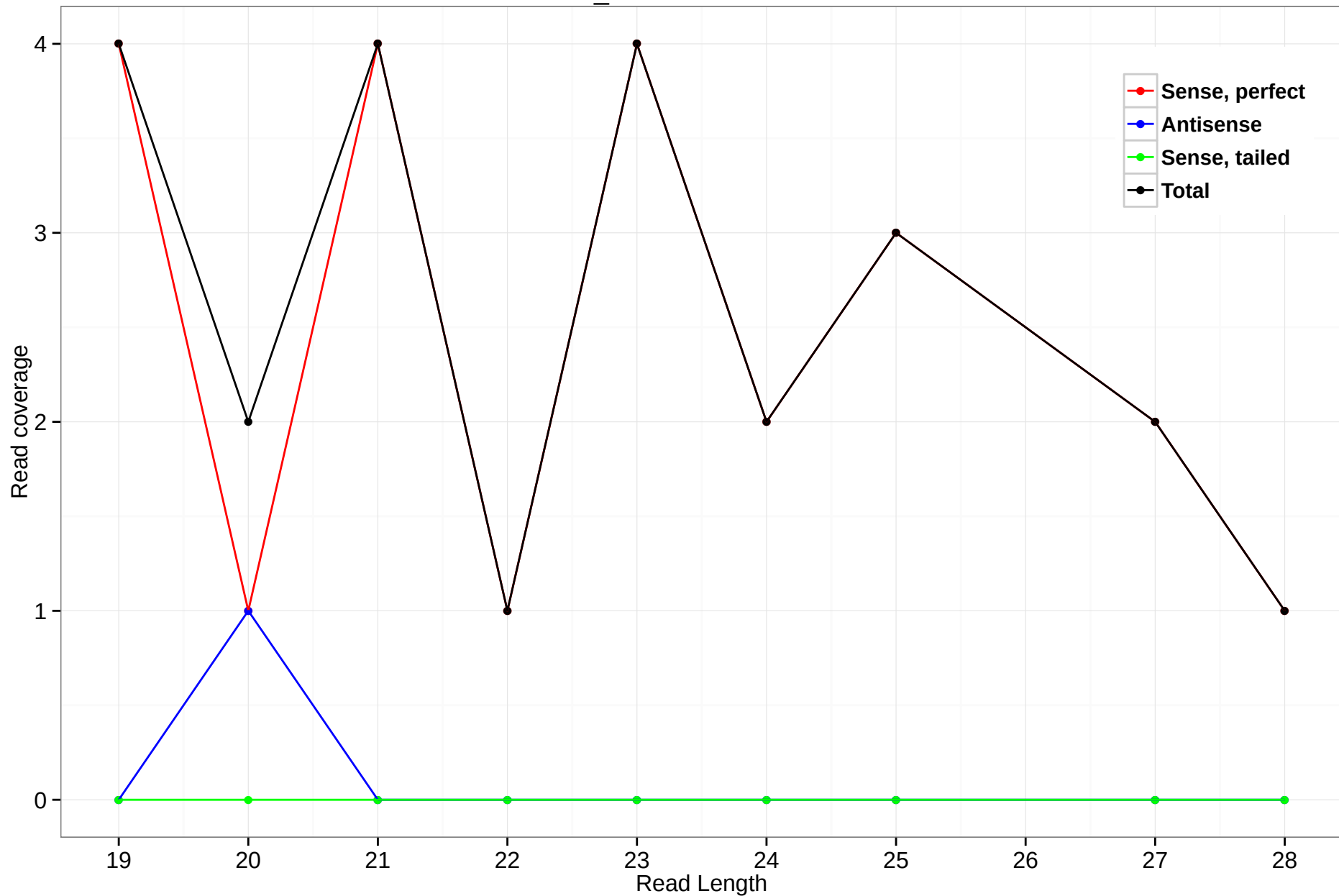
scaffold_4845:5592908-5593074
