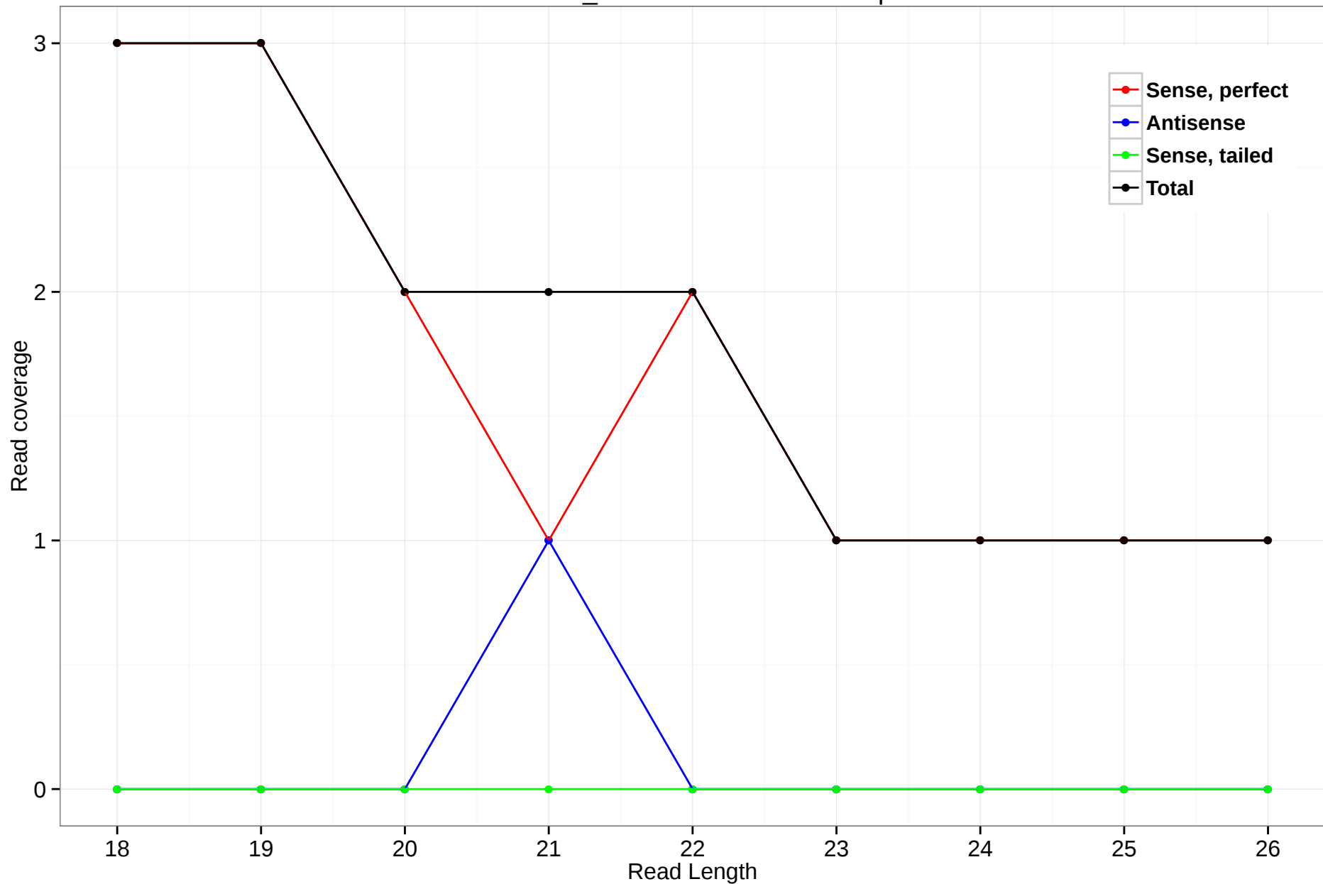
scaffold_4845:557000-963346.5p
