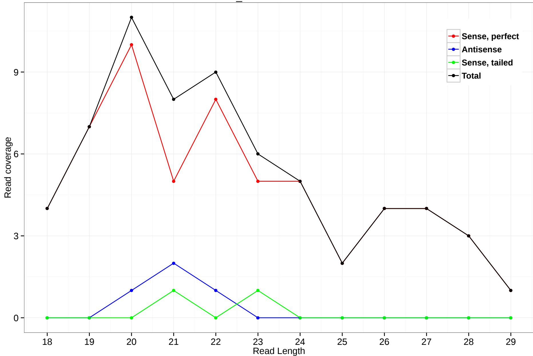
scaffold_4845:4752994-4753155
