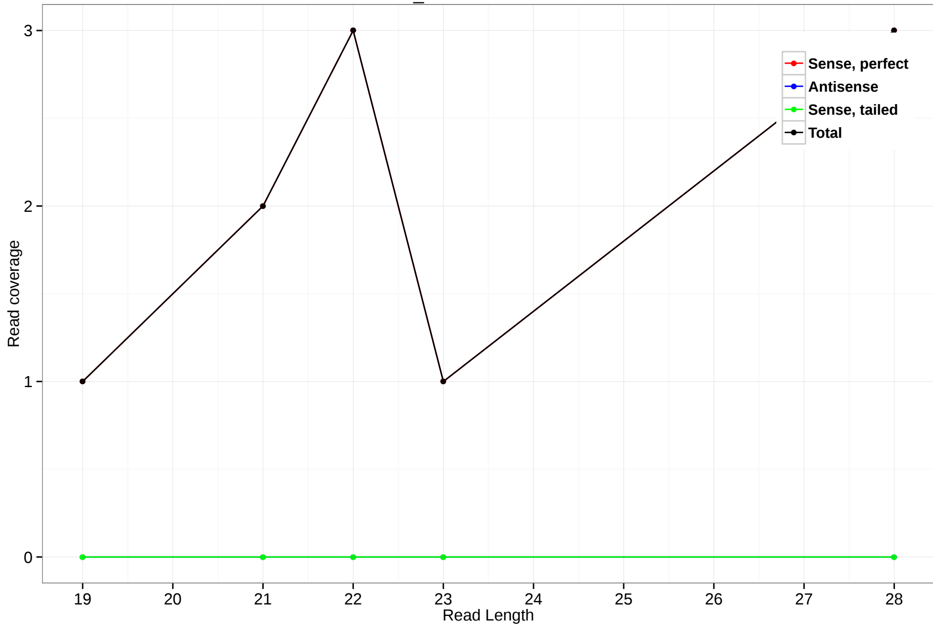
scaffold_4845:4363949-4364133
