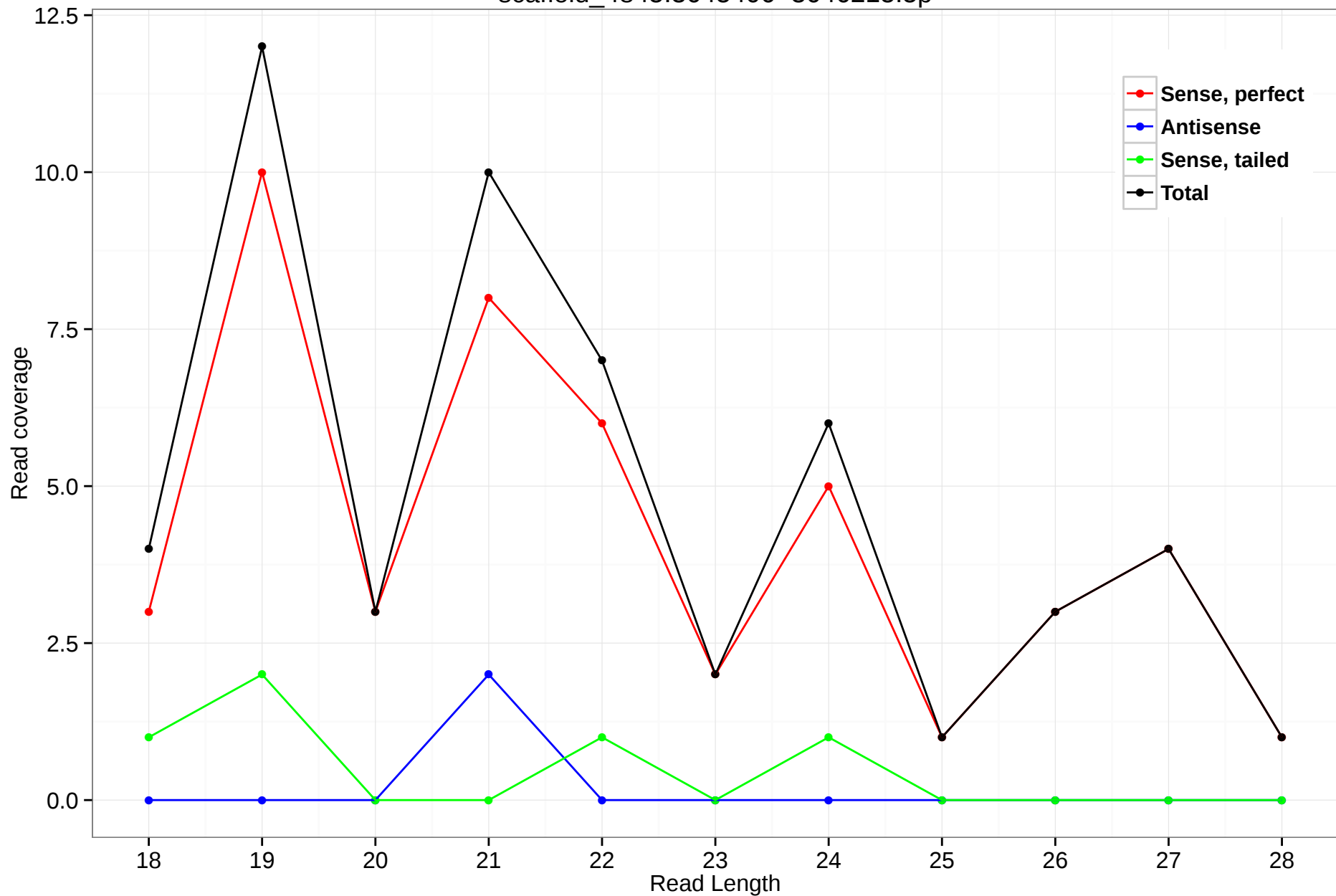
scaffold_4845:3645406-3646215.5p
