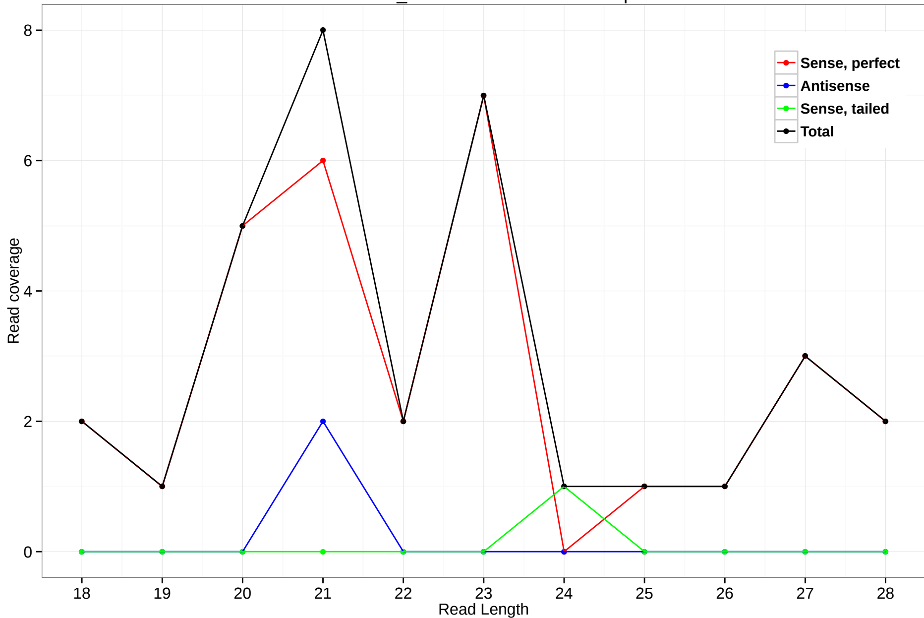
scaffold_4845:3645406-3646079.3p
