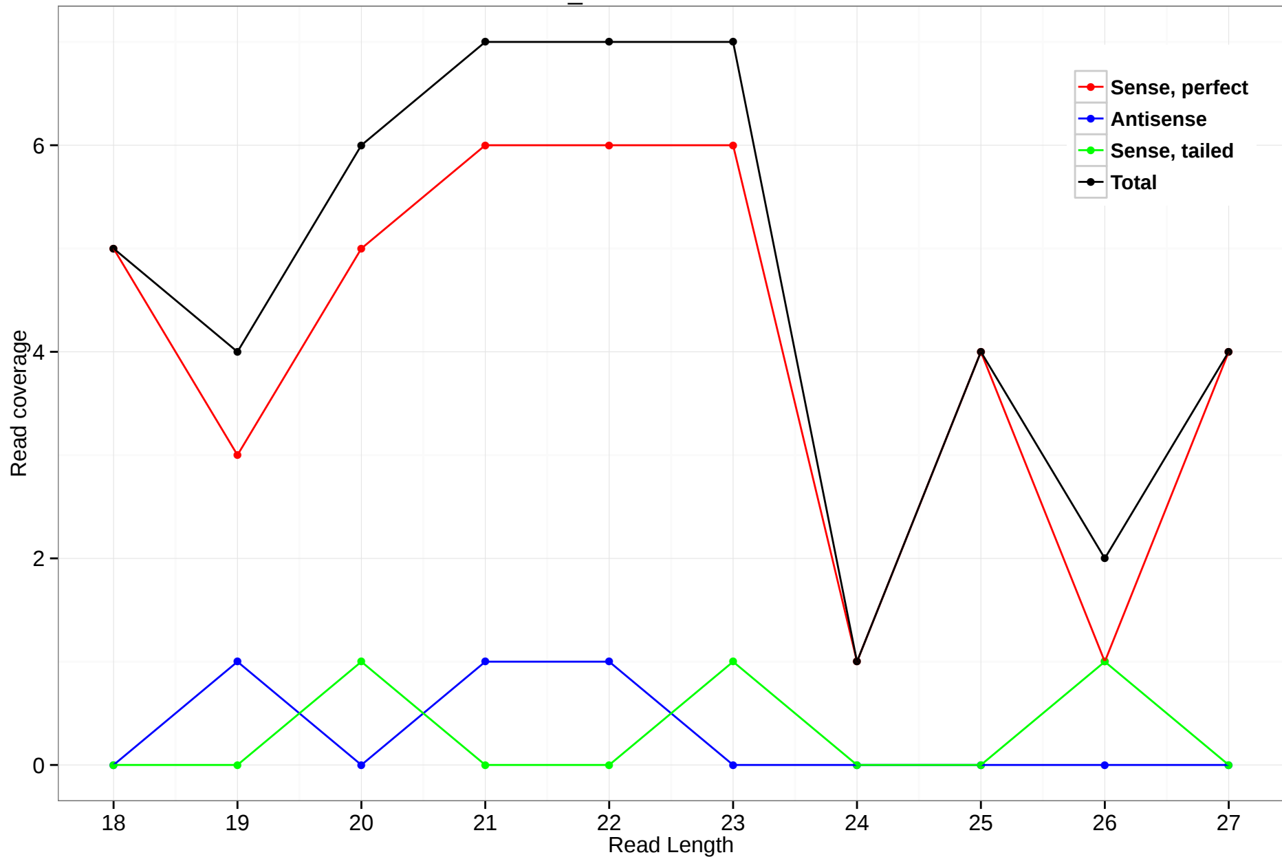
scaffold_4845:3645031-3645283
