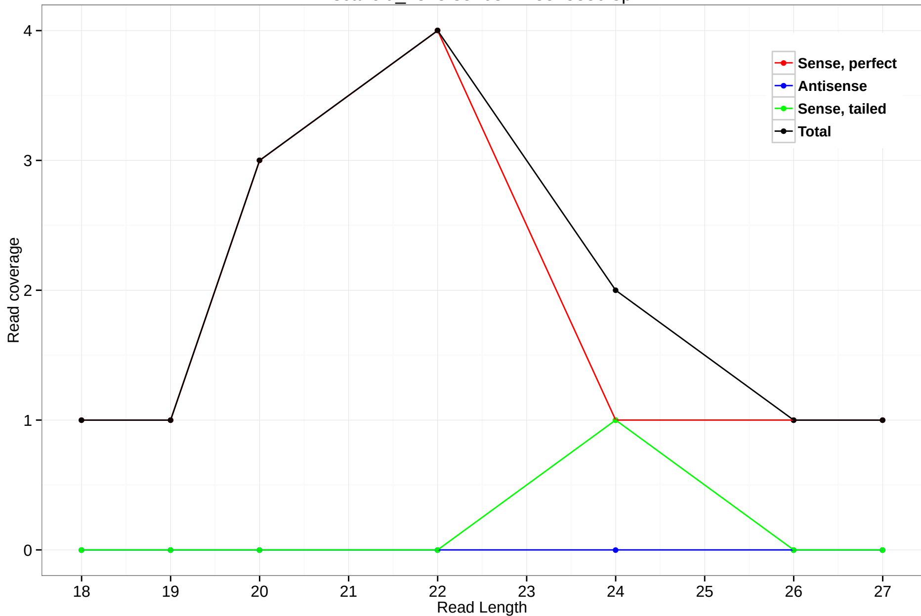
scaffold_4845:3570847-3575350.3p
