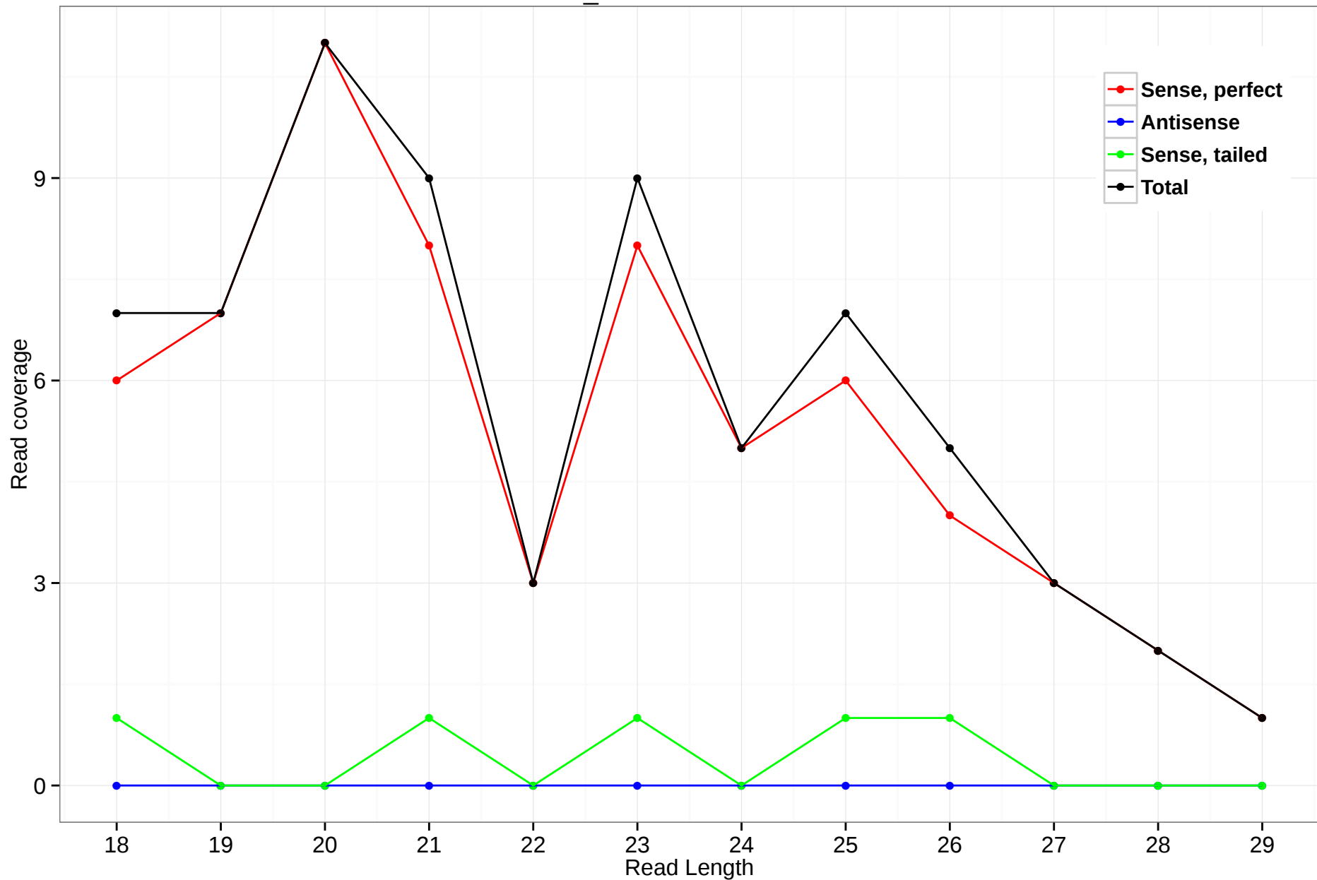
scaffold_4845:3349440-3349729
