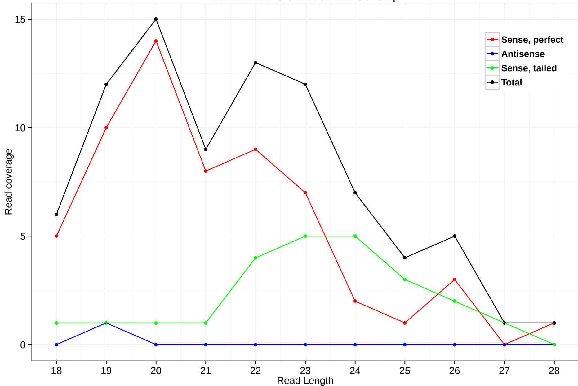
scaffold_4845:3328088-3329333.5p
