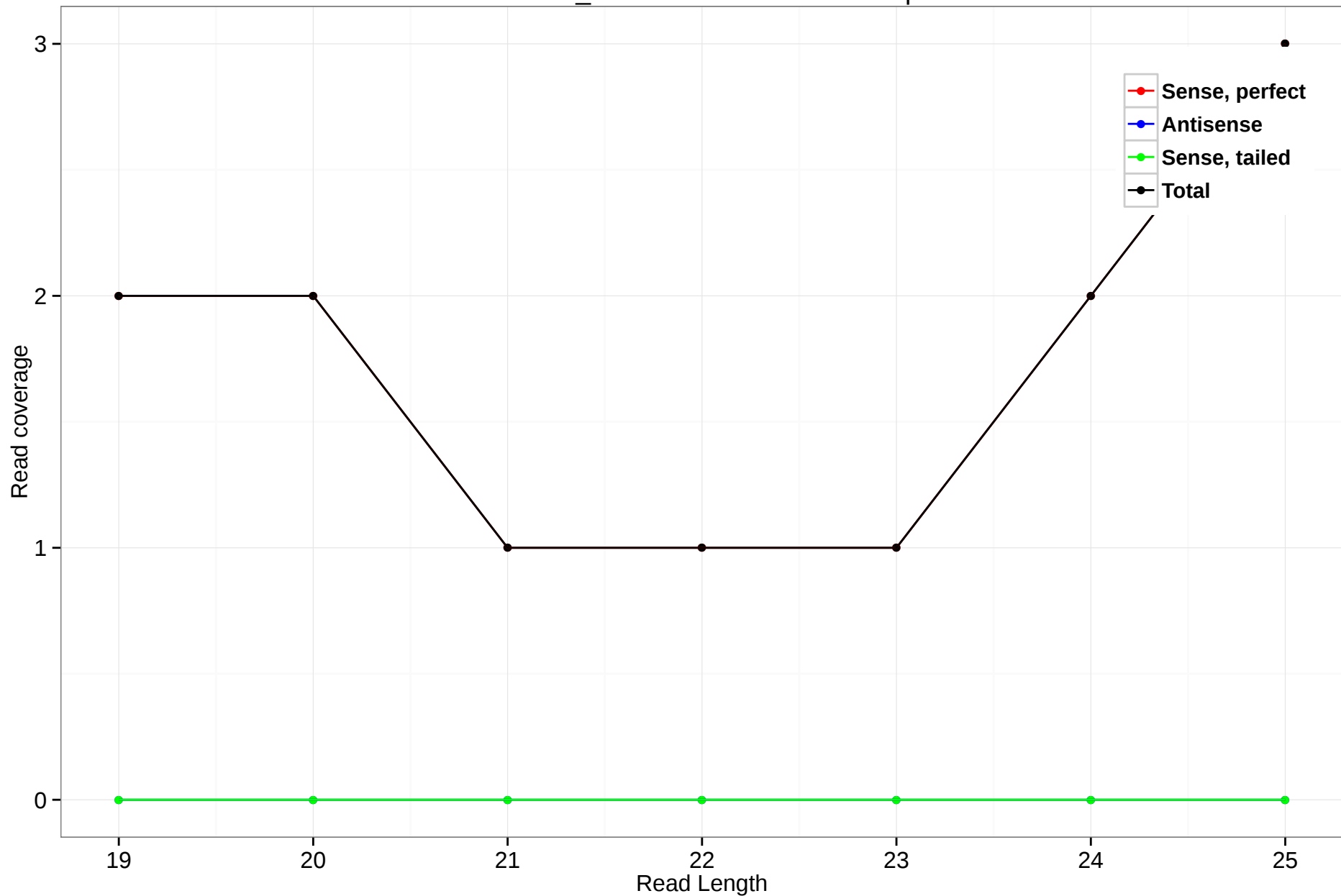
scaffold_4845:3219990-3221689.3p
