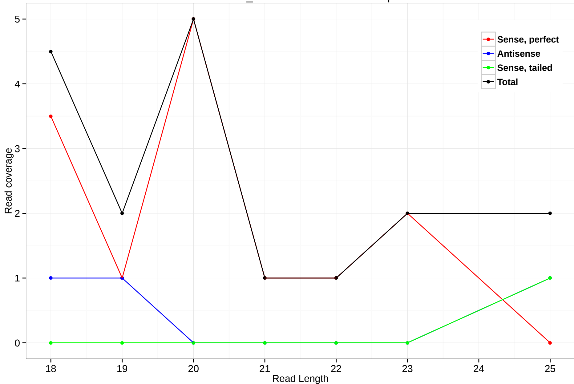
scaffold_4845:3188655-3189756.5p
