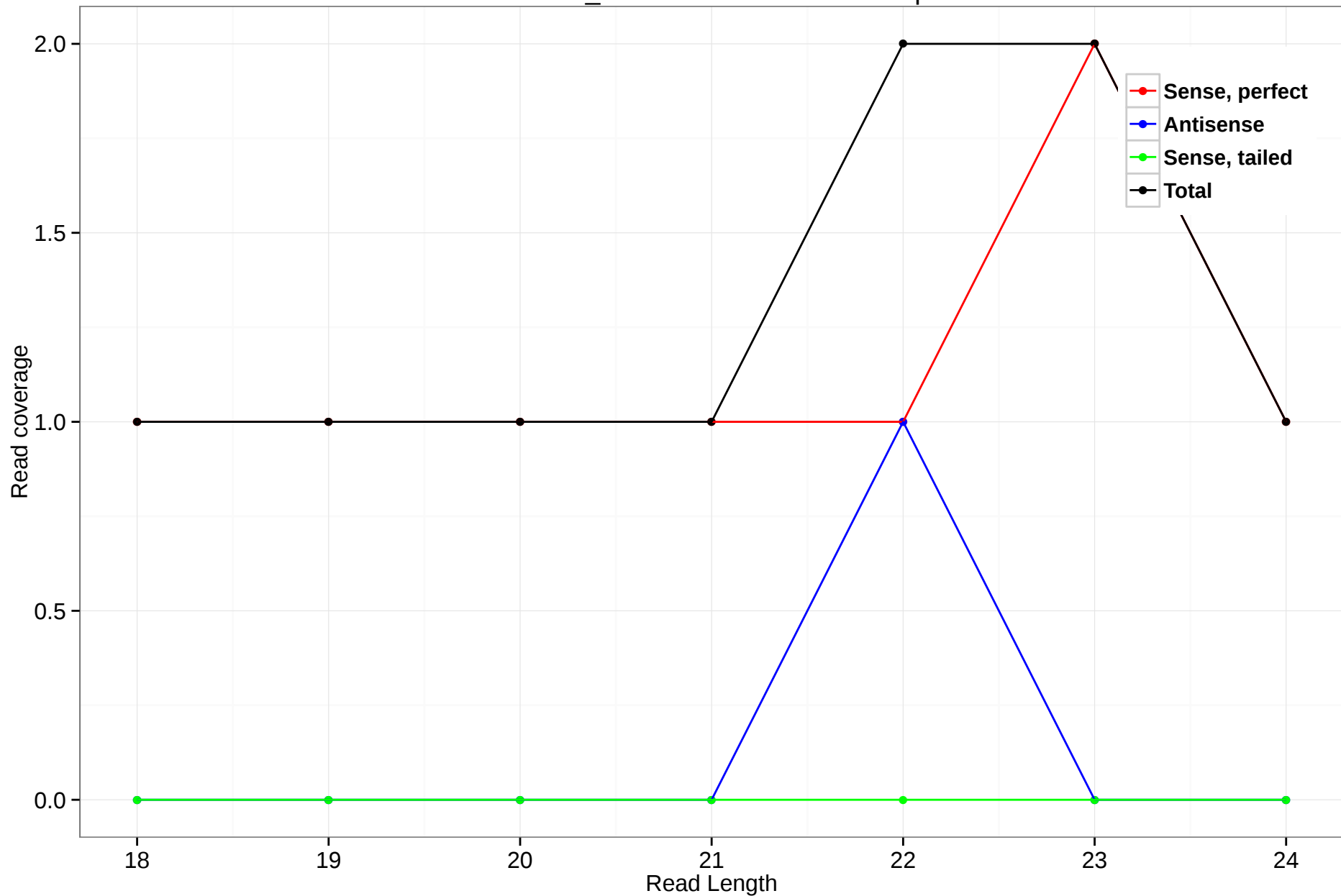
scaffold_4845:3143657-3144401.5p
