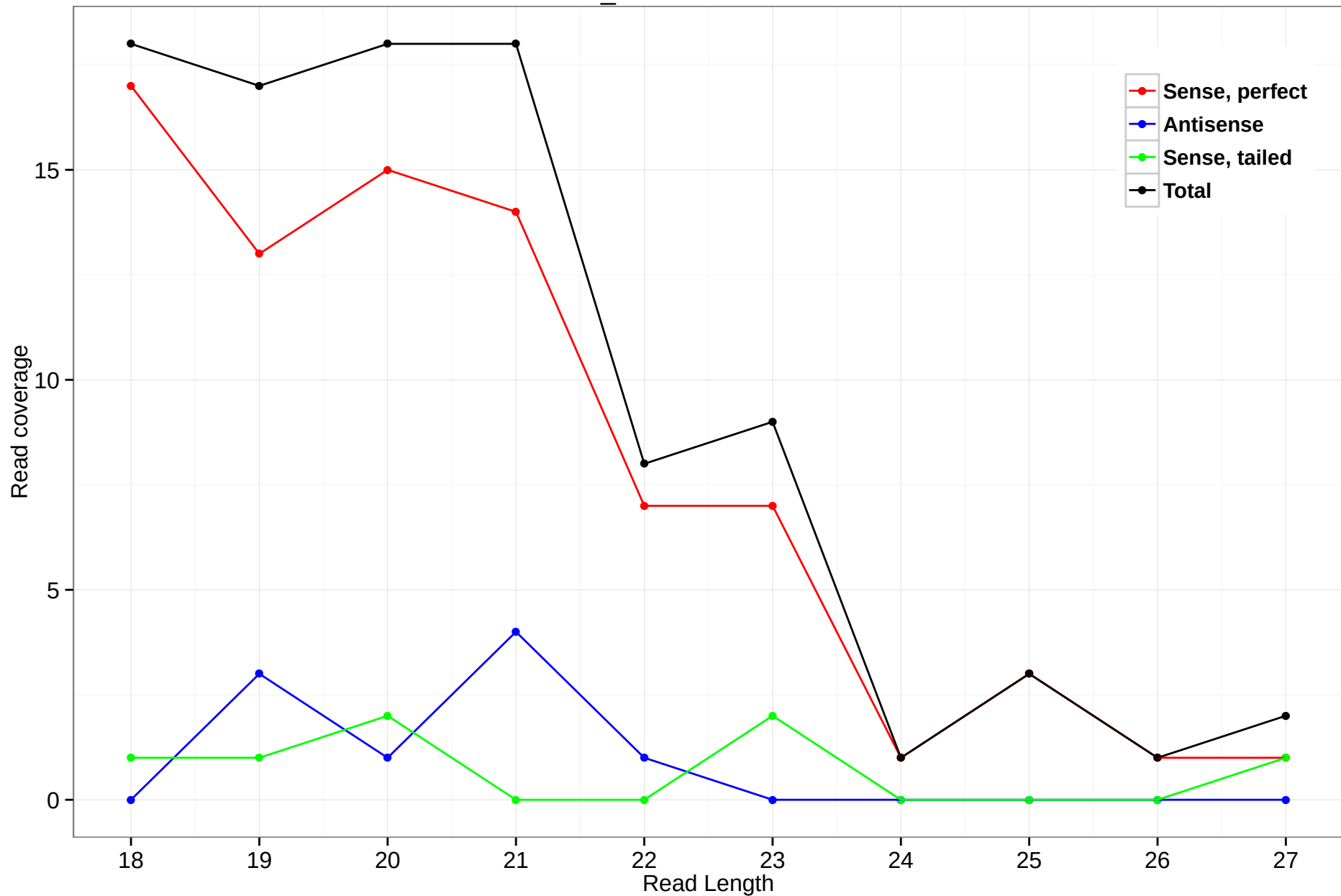
scaffold_4845:3012475-3012647
