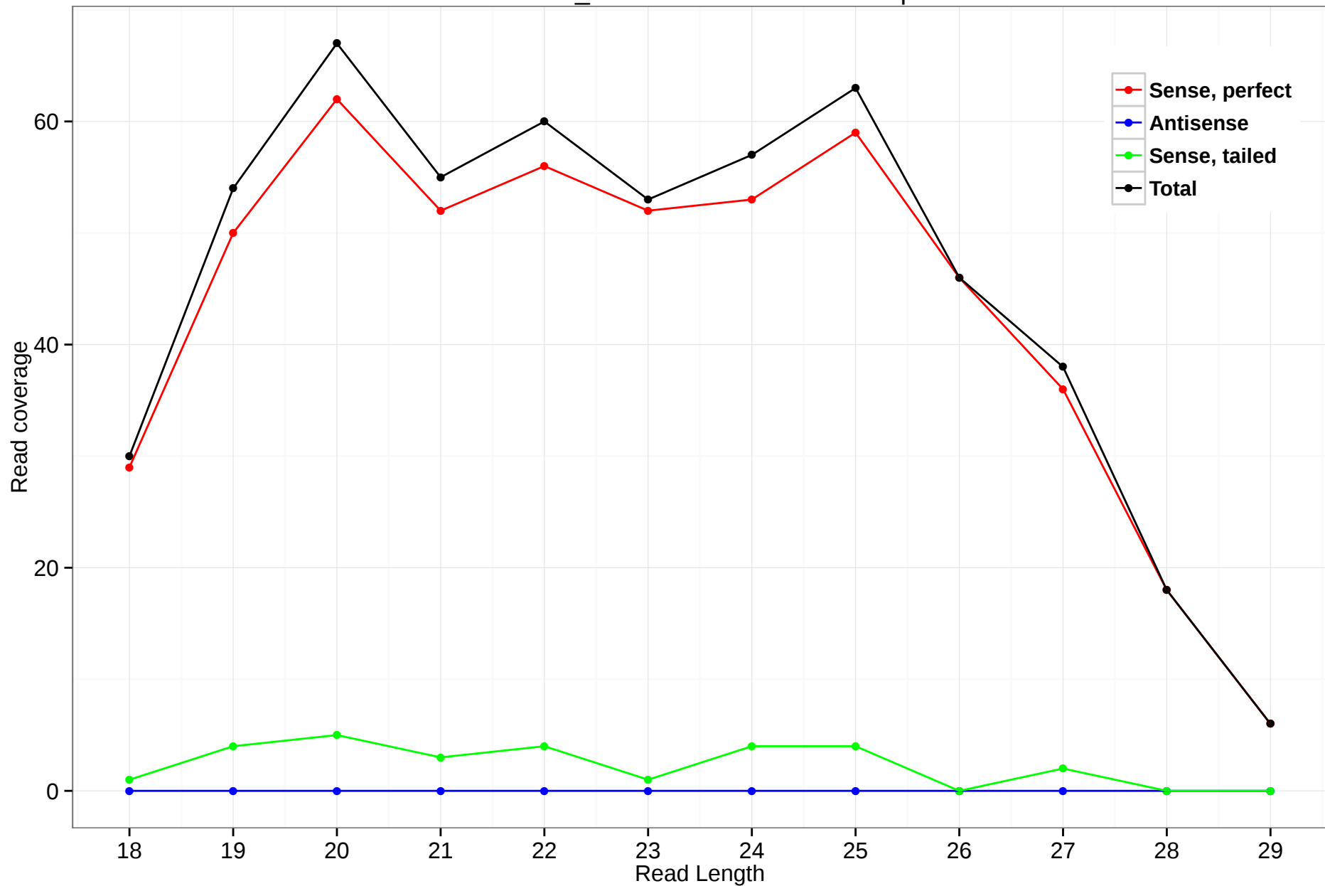
scaffold_4845:2844570-2845317.5p
