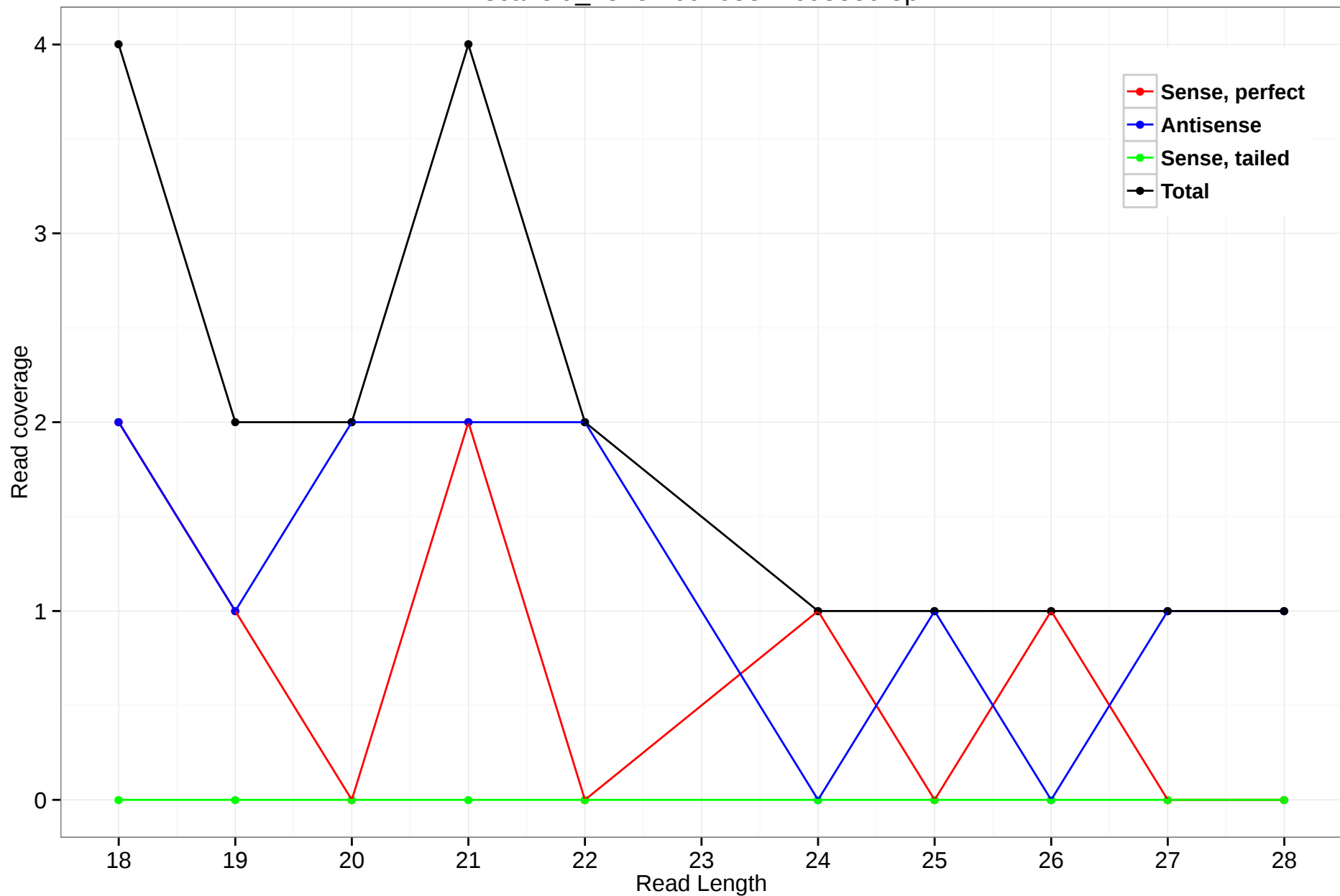
scaffold_4845:2691688-2695859.3p
