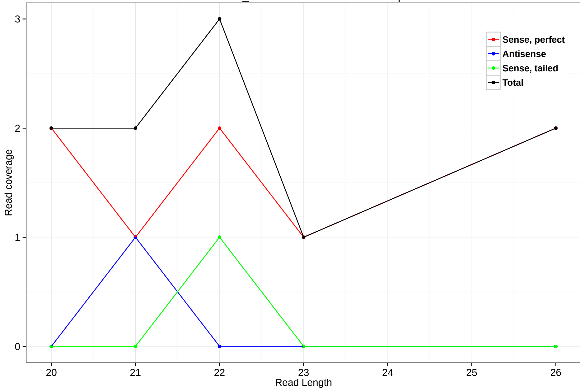
scaffold_4845:22273442-22274266.5p
