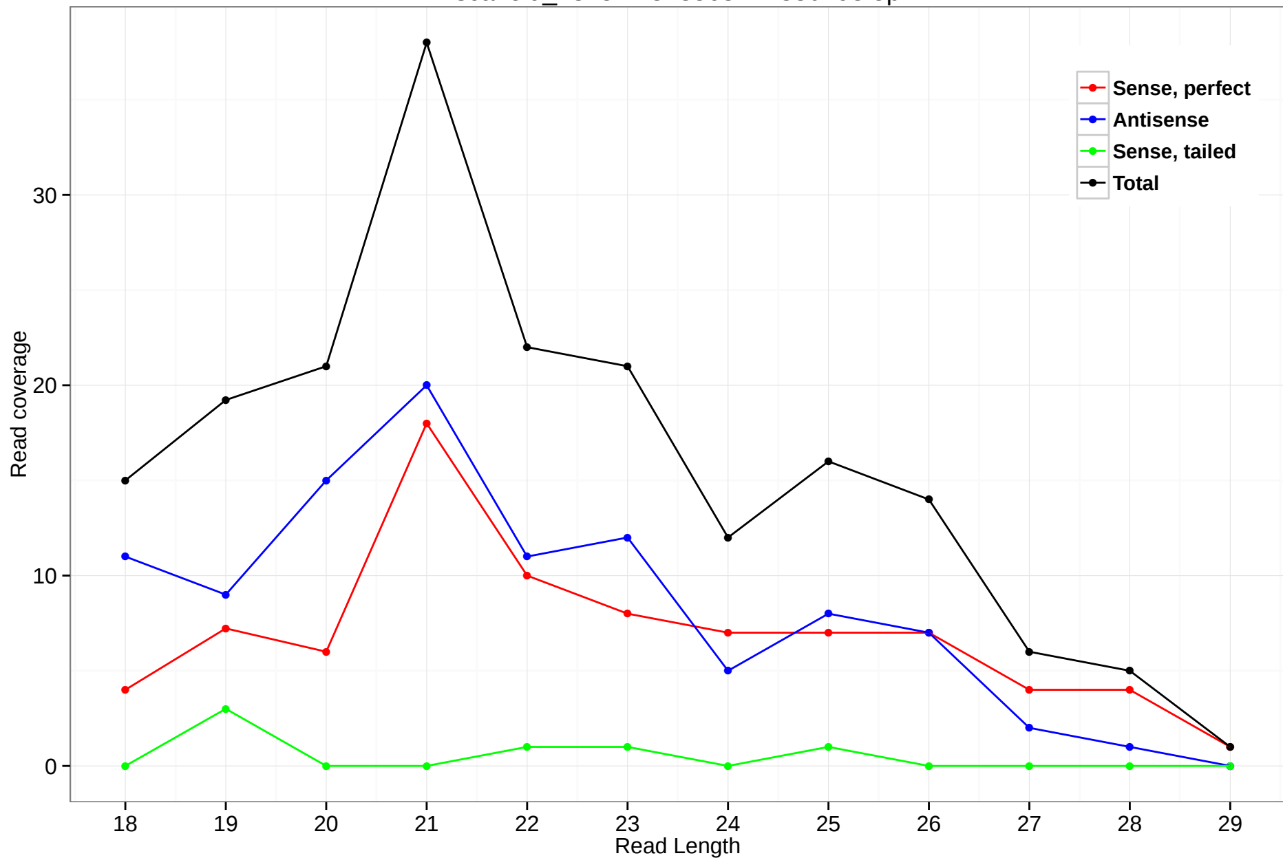
scaffold_4845:21828563-21830198.5p
