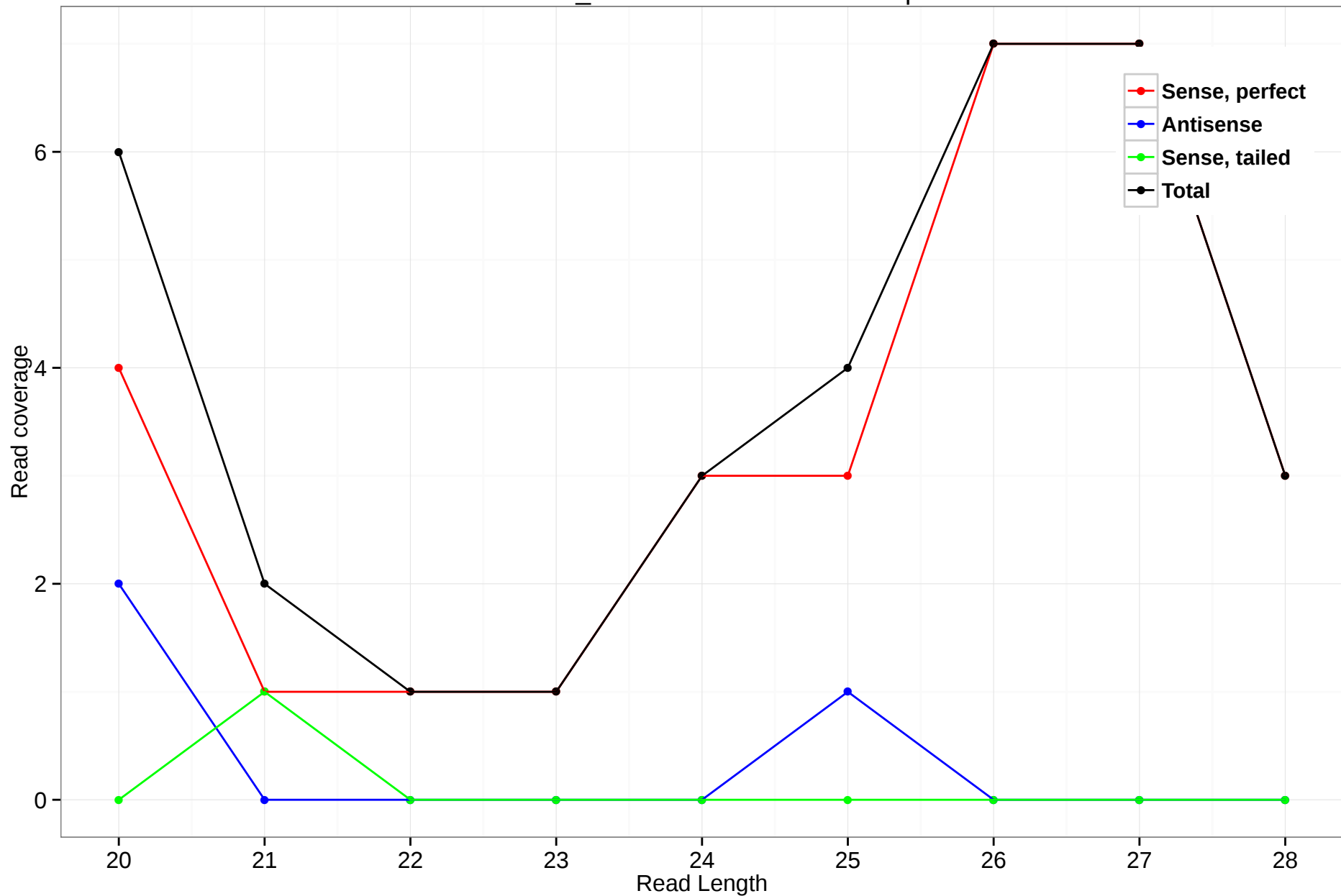
scaffold_4845:2180303-2192972.3p
