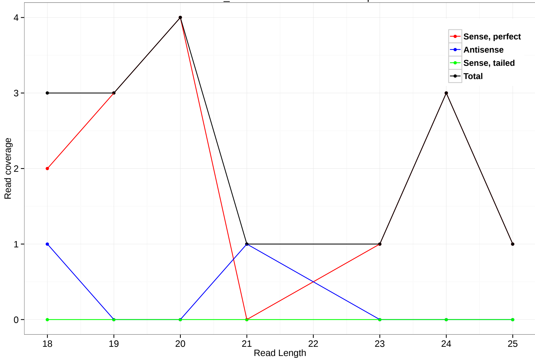
scaffold_4845:21200610-21201251.5p
