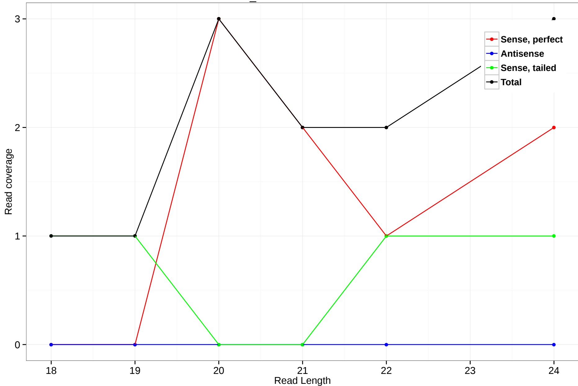
scaffold_4845:20924806-20924979
