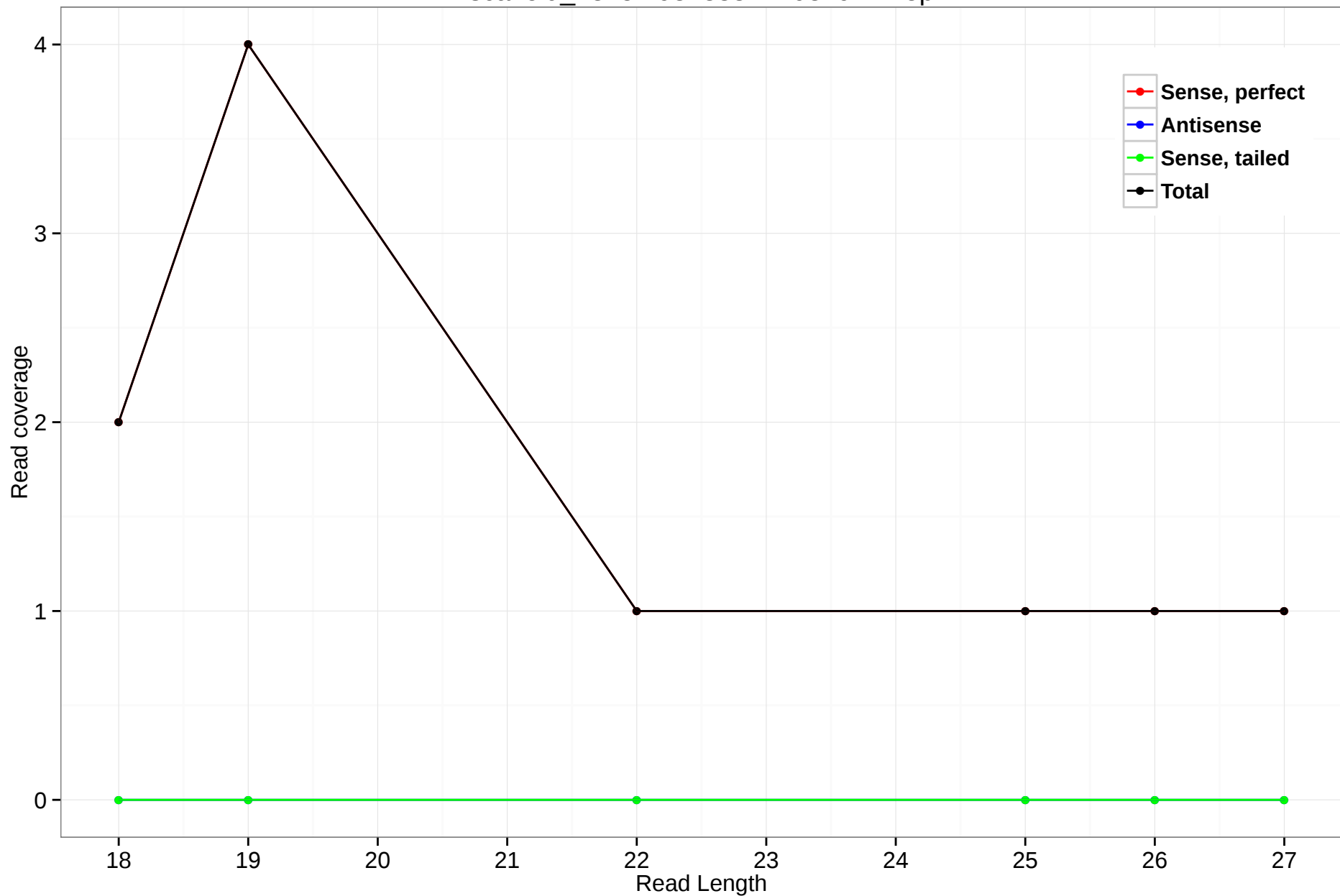
scaffold_4845:19848332-19849411.5p
