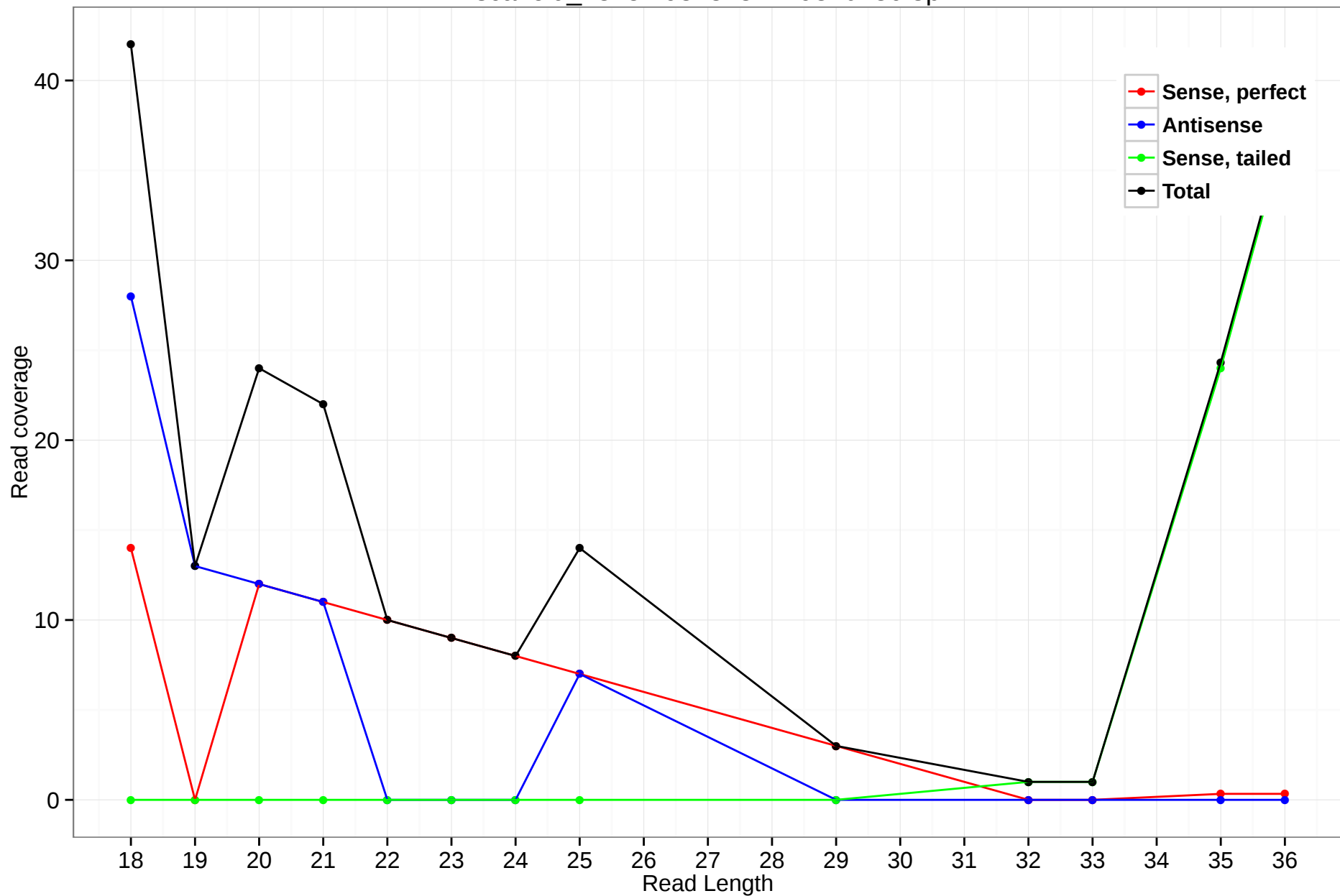
scaffold_4845:19818182-19820786.3p
