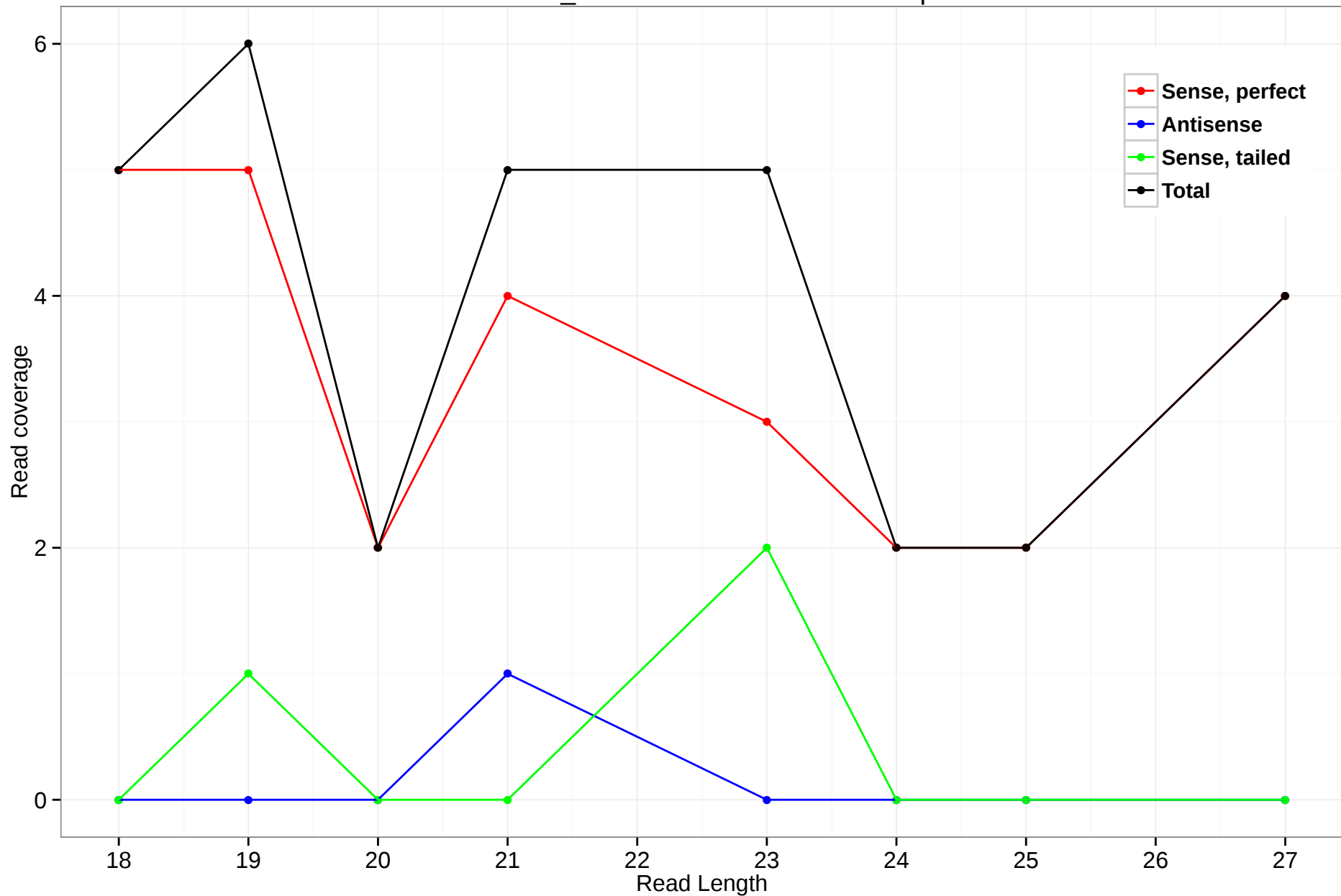
scaffold_4845:19791317-19793547.5p
