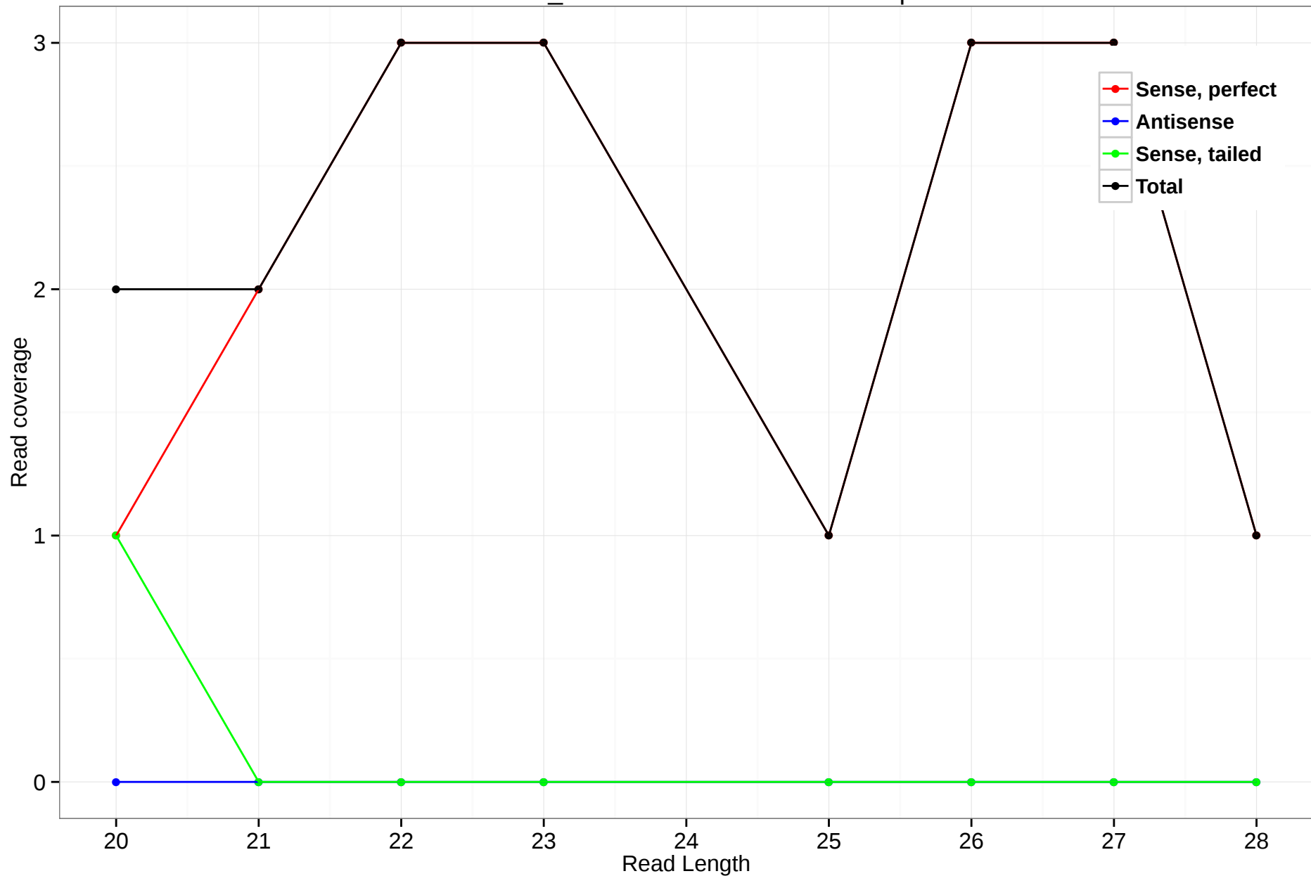
scaffold_4845:19352717-19353930.5p
